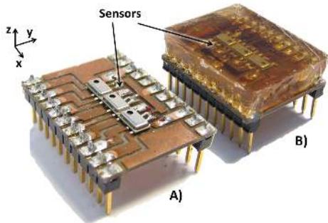
Figure 4. Sensors layout in the experimental setup. A: Before cast. B: In 6mm rubber.
