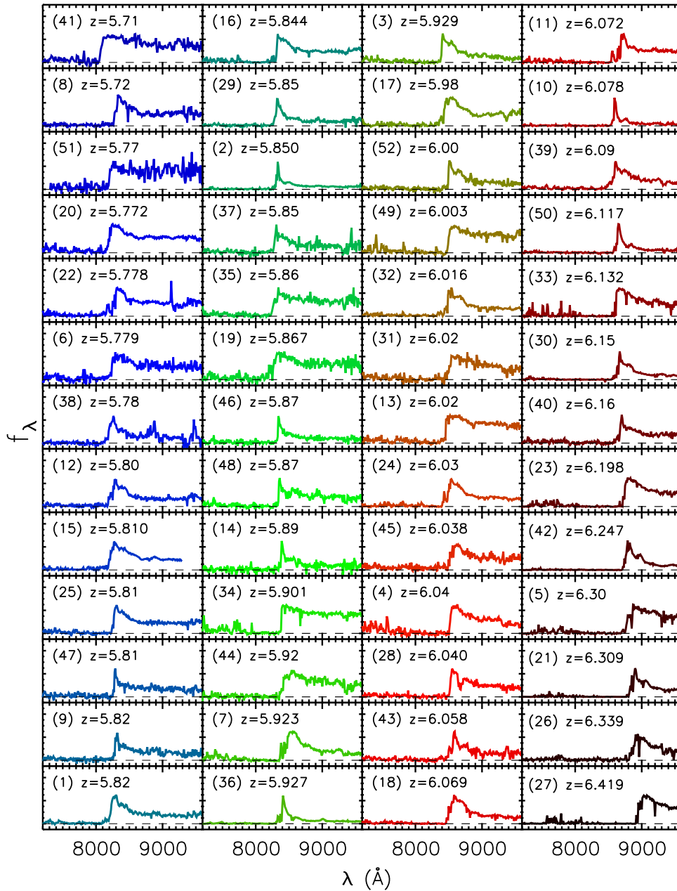
Figure 12. Optical spectra of the 52 SDSS quasars at z \sim 6 . See the main text for details.
