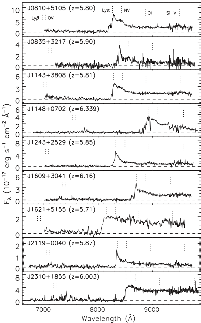
Figure 2. Optical spectra of the nine newly discovered quasars. The spectrum of J2310+1855 was taken with the LBT MODS. The other spectra were taken with the MMT RCS. The dashed lines indicate the zero flux level for each spectrum. Each spectrum has been scaled to match the corresponding z -band magnitude in Table 1, thereby placing it on an absolute flux scale.
