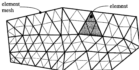
FIGURE 43. The recourse to field reconstruction for the discretization of the constitutive relations requires the definition of an additional geometric structure, in addition to the primary and secondary meshes, namely, an element mesh for each field to be reconstructed. Here each object of the new mesh is obtained as the union of cells of the primary or secondary mesh, but more general geometric structures not based on the two preexisting meshes can be used as well.
