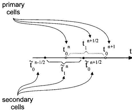
FIGURE 34. Reference discretization of the domain in time.
