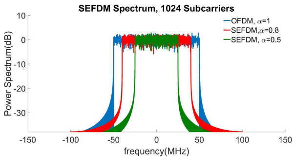
Figure 1. Illustrative spectra of SEFDM and OFDM signals.
