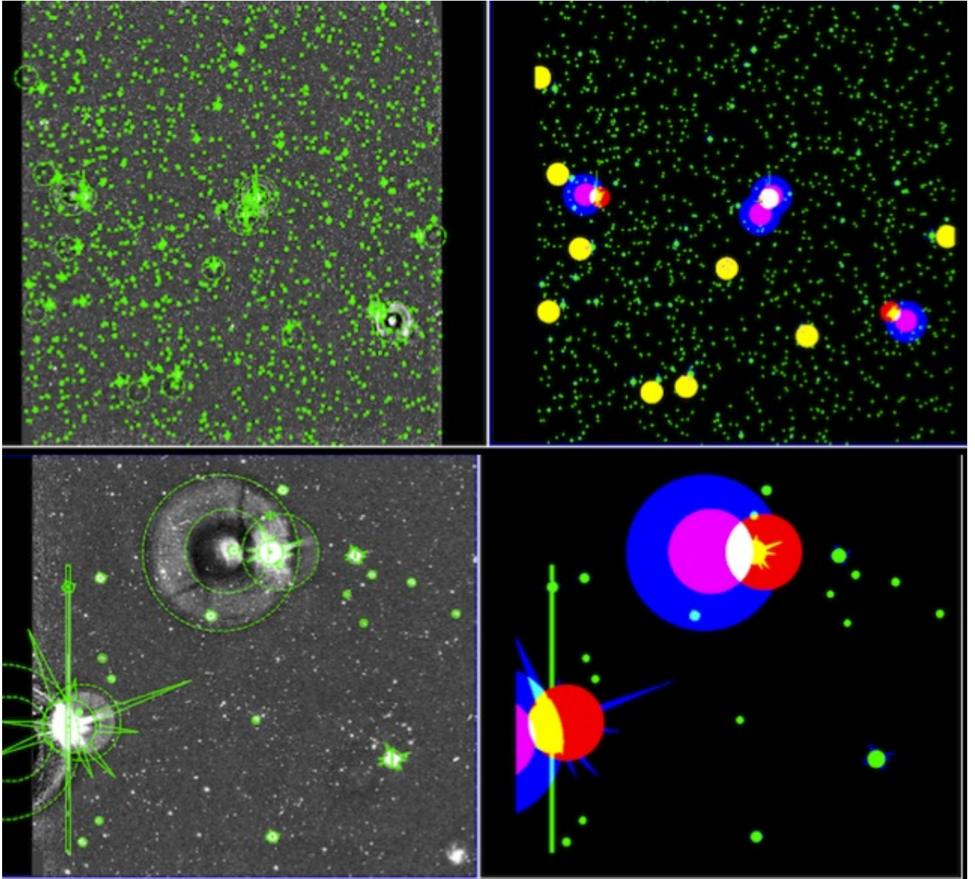
Fig. 7. Examples of a P_{v1.0} mask. Top left: thumbnail of a KiDS stacked image with several bright stars; critical areas detected by P_{v1.0} are overplotted with green outlines (region format). Top right: FLAG image corresponding to the image shown on the top left , with different colours corresponding to the pixel value with the binary flag values summed. Bottom panels: as top panels , but for a small area in a (different) KiDS stacked image.
