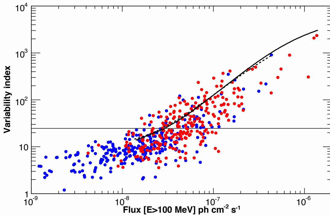
Fig. 19.— Variability index versus flux for FSRQs (red) and BL Lacs (blue) in the clean sample. The curves display the evolution of the variability index for the FSRQ 3C 454.3 (solid) and the BL Lac object AO 0235+164 (dashed) that would be observed for the same temporal variation but lower mean fluxes.
