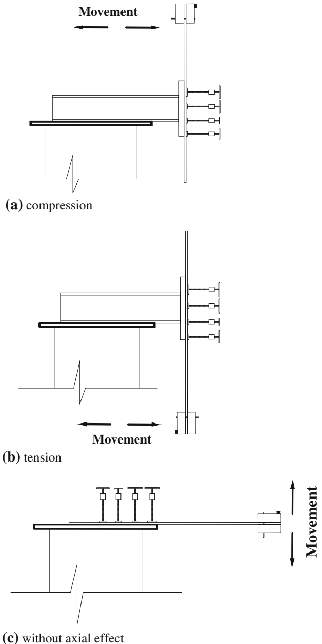
Fig. 3 Positions adopted in the tests
