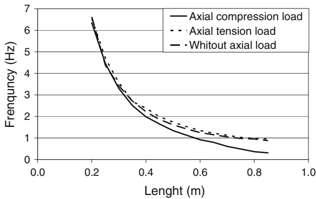
Fig. 6 Influence of a normal force on the experimental frequencies
