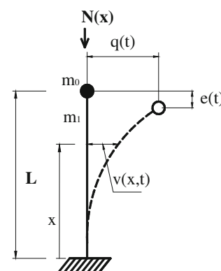
Fig. 1 Parameters for developing the mathematical model
