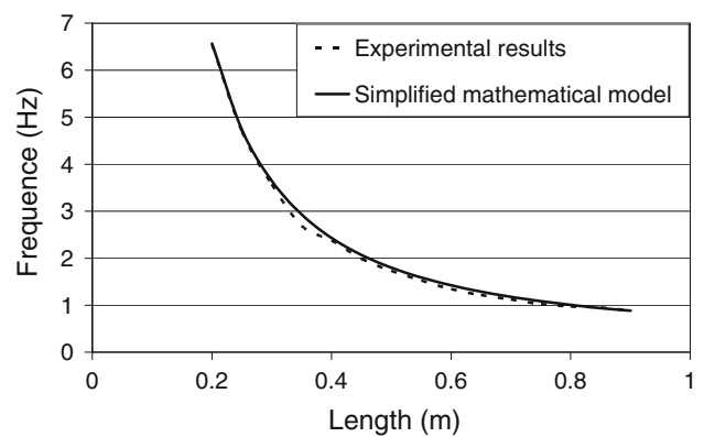
Fig. 8 Tension force: experimental results and mathematical model
