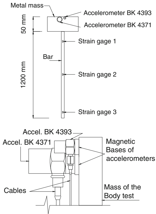
Fig. 2 Instrumentation of the test sample and the details of the accelerometer settings
