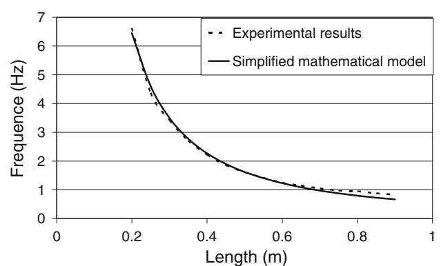
Fig. 9 Without normal force: experimental results and mathematical model
