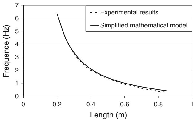
Fig. 7 Compressive force: experimental results and mathematical model
