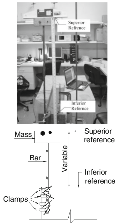
Fig. 4 Inferior reference length of the models
