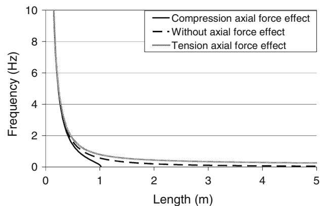
Fig. 5 Numerical simulation of the influence of the axial force
