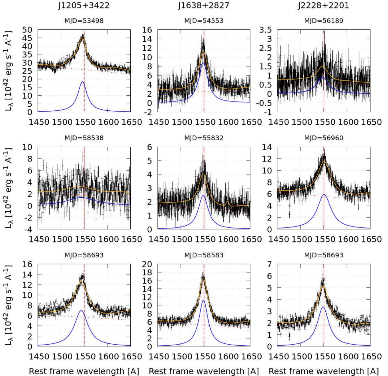
Figure 5. Observed spectra and best-fitting models of the CIV spectral region. The solid blue line is the Lorentzian profile fit to the CIV emission line. The long-dashed red line is the continuum fit, with the solid orange line giving the overall fit. The short-dashed vertical lines give the rest wavelengths of the CIV doublet.
