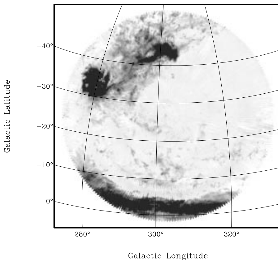
Figure 3 —Peak intensity map of a 2400\text{ deg}^2 region centred upon the South Celestial Pole, including the region shown in Figure 2. The velocity range encompassed here is v_{\text{lsr}} = 85\text{--}400\text{ km s}^{-1} . The Large and Small Magellanic Clouds, the Magellanic Bridge and the beginning of the Magellanic Stream are shown at the top of the figure. The Galactic Plane, which extends out to 120\text{ km s}^{-1} in the direction (\ell, b) = (300^\circ, 0^\circ) (Burton 1988), is seen at the bottom of the figure.
