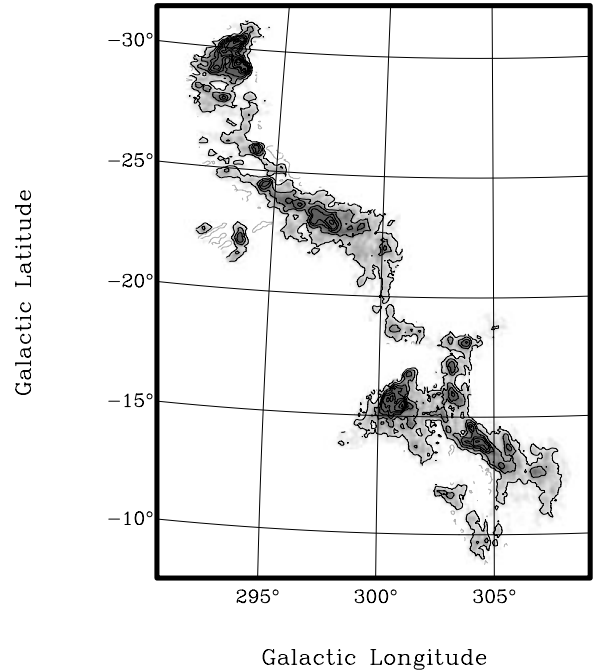
Figure 4 —A detailed view of the Leading Arm at the channel centred upon v_{\text{lsr}} = 323 km s -1 . Contours are from 10–90% of the brightness temperature maximum ( T_{\text{B}} = 0.88 K). The link between the Magellanic System and the strong emission features at (\ell, b) = (297^\circ, -24^\circ) and (\ell, b) = (302^\circ, -16^\circ) is not visible in the earlier data of Mathewson & Ford (1984) (their Figure 2) or Morras (1982), due to their sparse spatial sampling. The total HI mass of the Arm is \sim 1 \times 10^7 M_{\odot} . See Putman et al. (1998) for further details.
