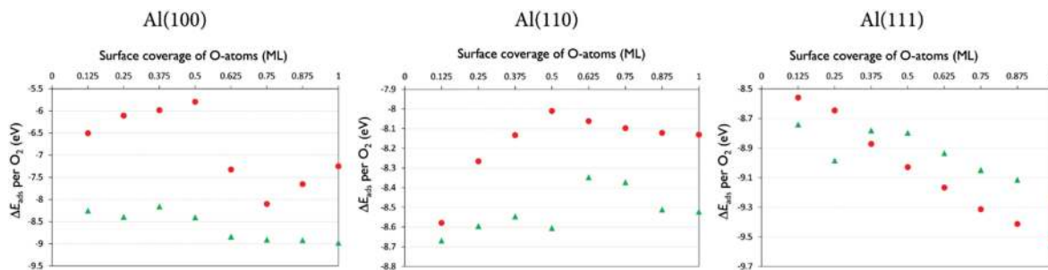
Fig. 5 Adsorption energies per dissociating \text{O}_2 molecule ( \Delta E_{\text{ads}} (eV)) that gives rise to the corresponding coverage of O-atoms at the surfaces (ML) for the two oxide growth modes here studied: clusters and stripes ( \blacktriangle ), homogeneous ( \bullet ).
