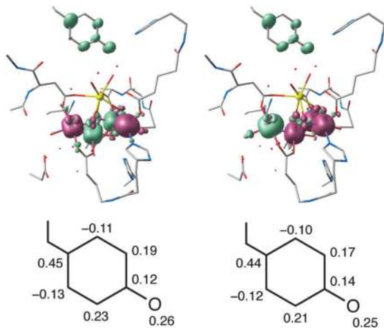
Fig. 4 Spin density maps and Mulliken spin populations on the tyrosyl fragment for models of the open cubane S_2^{A}Y_Z^* (left) and closed cubane S_2^{B}Y_Z^* (right) states of the OEC in their respective lowest-energy broken-symmetry spin configurations.
