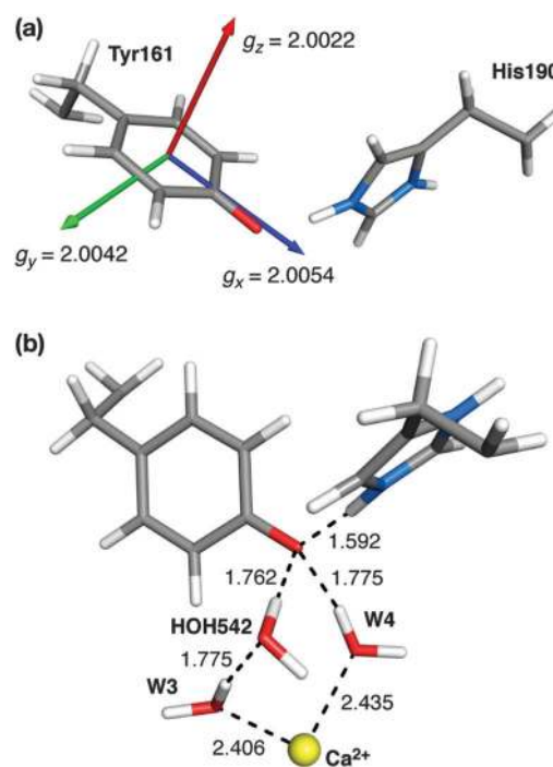
Fig. 7 (a) Orientation and components of the g-matrix for the S 2 B Y Z • state. (b) Water molecules involved in hydrogen bonding to Y Z • (distances, in Å, shown for the S 2 B Y Z • model).
