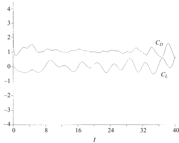
FIGURE 10. Variation of the drag and lift coefficients, C_D and C_L with t at R = 500 , S = \pi/2 and \alpha_m = 1.0 .
