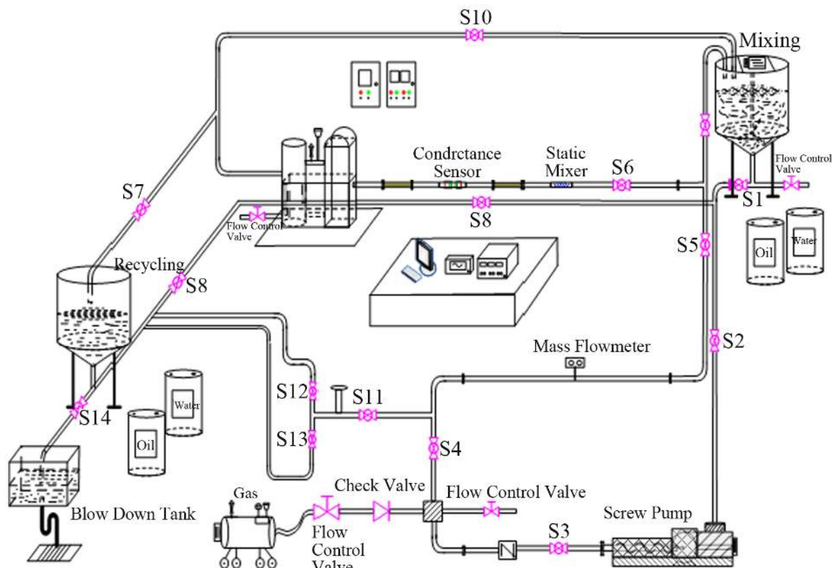
Figure 4. Experimental system.
