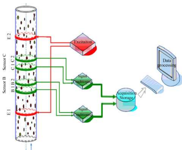
Figure 3. Conductance sensor measuring system.
