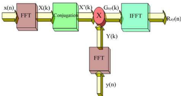
Figure 2. The correlation function calculation in frequency domain.
