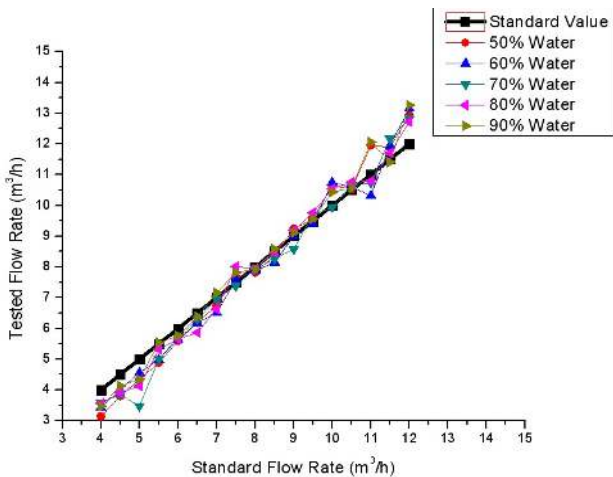
Figure 6. Tested flow rate and standard flow rate under various water fractions.
