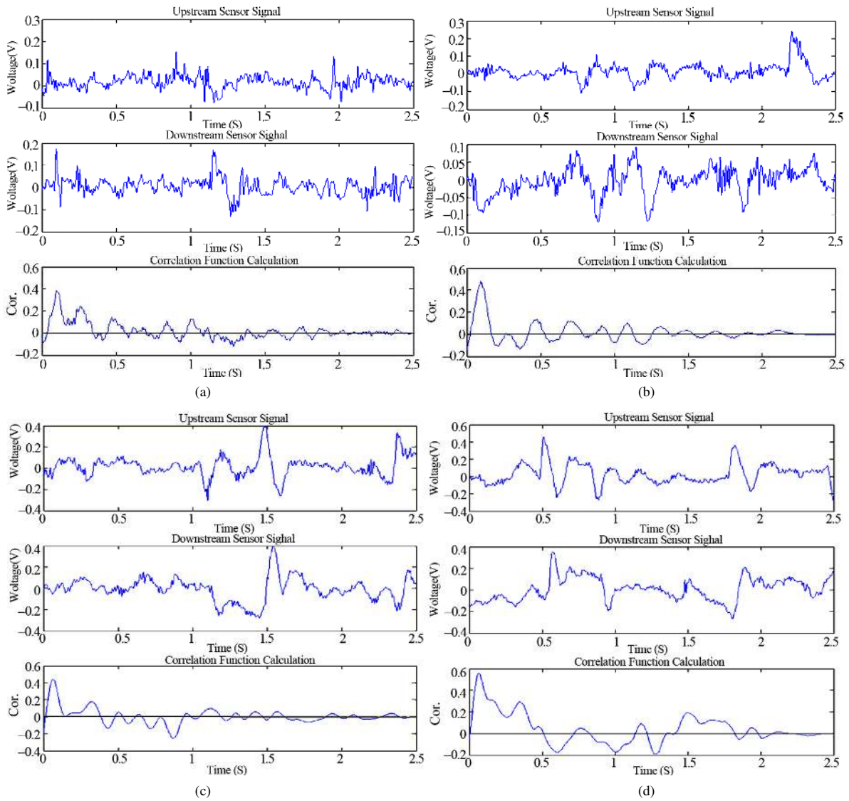
Figure 5. Flow signal waves and the results of the correlation operation.
