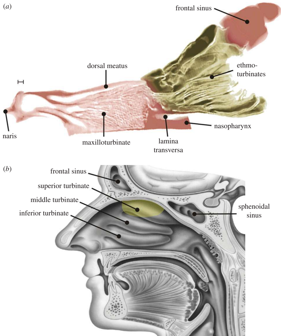
Figure 2. The canine olfactory recess. (a) A sagittal section of the canine nasal airway reveals a peripherally located olfactory recess excluded from the respiratory part of the nose by a bony horizontal plate, the lamina transversa . This anatomical feature is characteristic of keen-scented (macrosmatic) animals and influences olfactory airflow patterns and odorant transport. Scale bar 2.5 mm. (b) For comparison, a sagittal view of the human nasal airway demonstrates the absence of an olfactory recess in the human nose (courtesy Hornung 2006). Here, the delineation of the olfactory region is as illustrated by Lang (1989). As shown by Morrison & Costanzo (1990, 1992), the shift from respiratory to olfactory epithelium is not uniform or well defined, but rather is characterized as having a mixed and irregular boundary, where clusters of olfactory cells are found among non-olfactory cells. The olfactory region shown here corresponds to the approximate location of the olfactory epithelium. Yellowish-brown, olfactory region; pink, respiratory region.
