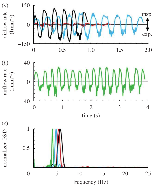
Figure 4. Experimental results from airflow measurements of canine sniffing. (a) Sample measurements for three dogs of widely different body size reveal the size-dependent variation of airflow rate for canine sniffing. Here, short sniffing bouts are shown that consist of a single burst of sniffs. (b) Longer bouts of sniffing typically contained multiple bursts of sniffs occurring in the 0.5–1.5 Hz range. (c) A plot of the normalized power spectral density (PSD) of sniffing calculated via a fast Fourier transform (FFT) of the time-dependent airflow rate data. For comparison, each PSD spectrum is normalized by the maximum PSD. Red lines, Pomeranian (6.8 kg); green lines, sheltie–husky mix (14.5 kg); blue lines, German shepherd (34.5 kg); black lines, Labrador retriever (52.9 kg).
