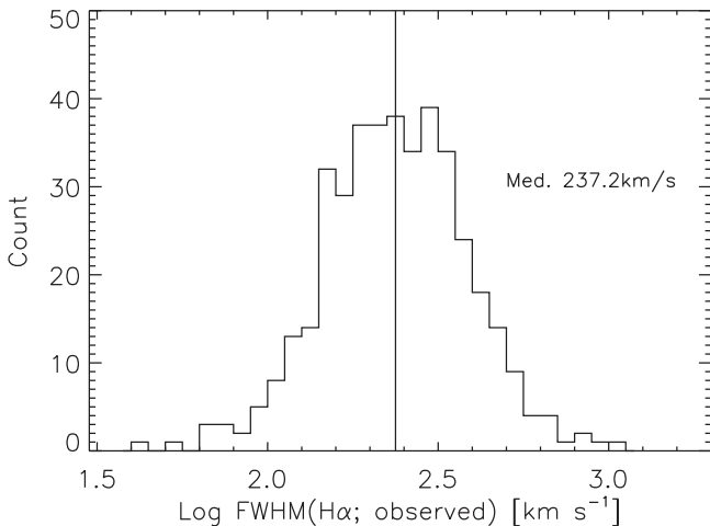
Figure 23. Distribution of the observed log FWHM of the H \alpha line (units of km s ^{-1} ).
