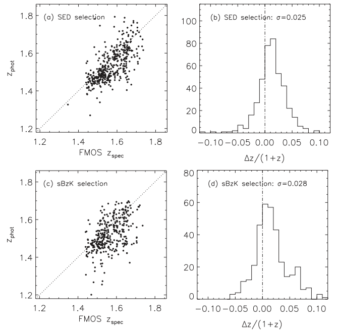
Figure 21. Comparison of spectroscopic and photometric redshifts. The top two panels are based on the SED-selected sample with the latest photometric redshifts (Ilbert et al. 2013). The bottom two panels make the same comparison using the sBzK sample and photometric redshifts derived prior to the availability of the UltraVISTA photometry. For both histograms, the quantity on the abscissa is (z_{\text{spec}} - z_{\text{phot}})/(1 + z_{\text{spec}}) with the standard deviation, including the clipping of 5\sigma outliers, of the distribution given in the respective panel for each distribution.
