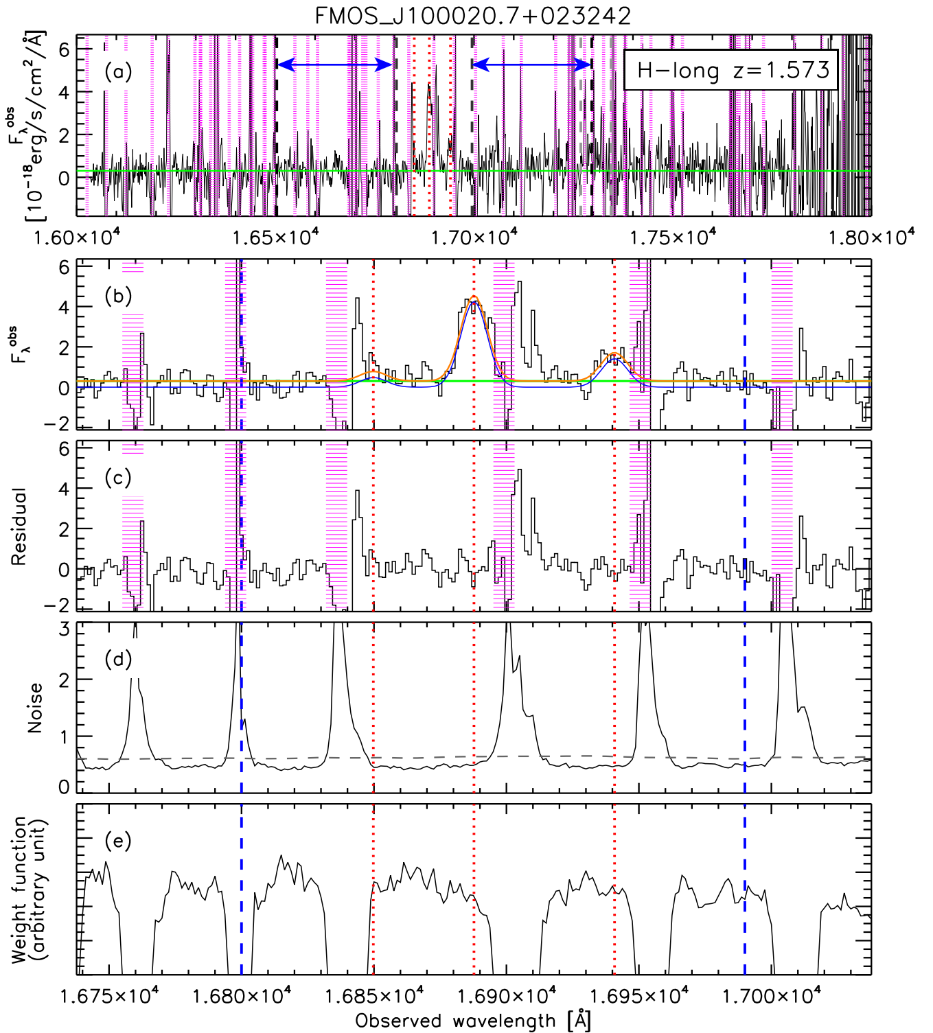
Figure 11. Example spectrum of a galaxy at z = 1.573 with a significant detection of H\alpha and [N\text{ II}]\lambda 6585 as indicated by the vertical dotted lines (red). Individual panels are as follows: (a) entire observed spectrum with regions impacted by OH lines shown in magenta. Two blue arrows indicate the regions used to determine the continuum level by fitting a linear function shown in green. (b) Observed spectrum over a narrower spectral range and centered on H\alpha . The overall fit to the spectrum is indicated in yellow with the components marked in green (continuum) and blue (emission lines). (c) Residual after subtracting the best-fit function to the emission lines and continuum. (d) rms noise level and threshold (horizontal dashed line) for avoiding the wavelength range impacted by OH lines. (e) Weight function applied to each pixel for fitting both the continuum and emission lines.
