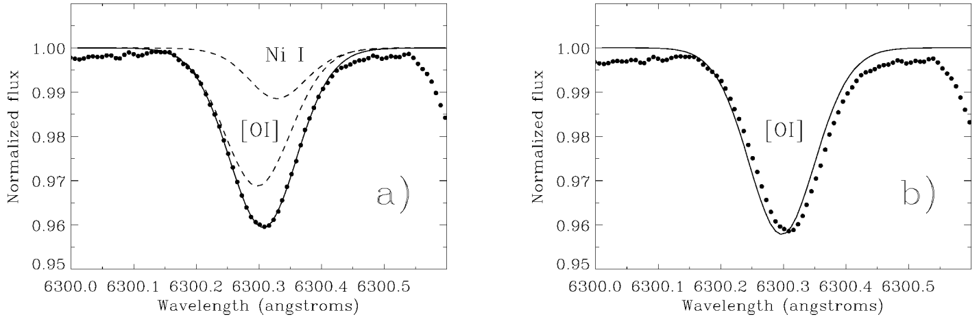
FIG. 1.—(a) Comparison between the observed ( filled circles ) and synthetic ( solid line ) profiles after the \chi^2 minimization. The individual calculations of the oxygen and nickel lines are also shown as dashed lines. (b) Best fit, assuming the observed feature is entirely produced by the oxygen forbidden line.
