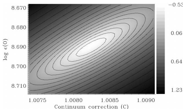
FIG. 2.—Contour and gray-scale plot showing the variation of the reduced \chi^2 as a function of the continuum level and the oxygen abundance, while keeping the nickel abundance constant. The plot uses logarithmic units, and therefore the units in the code bar of the gray scale are in decimal exponents.
