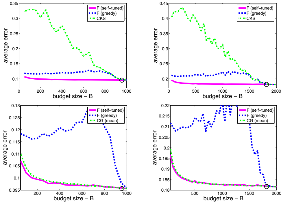
FIG. 6. The average online error of different budget algorithms as a function of the budget B on synthetic datasets with 5% label noise (left) and 10% label noise (right). The average accuracy of the Perceptron and its budget requirements for each problem are marked by a circle.
