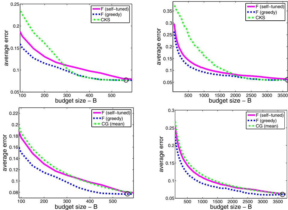
FIG. 4. The average online error of different budget algorithms as a function of the budget B on the USPS dataset (left) and the MNIST dataset (right). The online error of the Perceptron and its budget requirements for each problem are marked with a circle.
