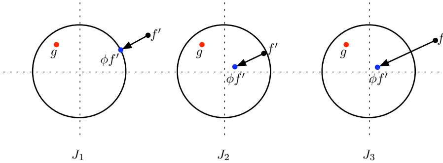
FIG. 1. A geometrical interpretation of the three hypothesis-shrinking cases.
