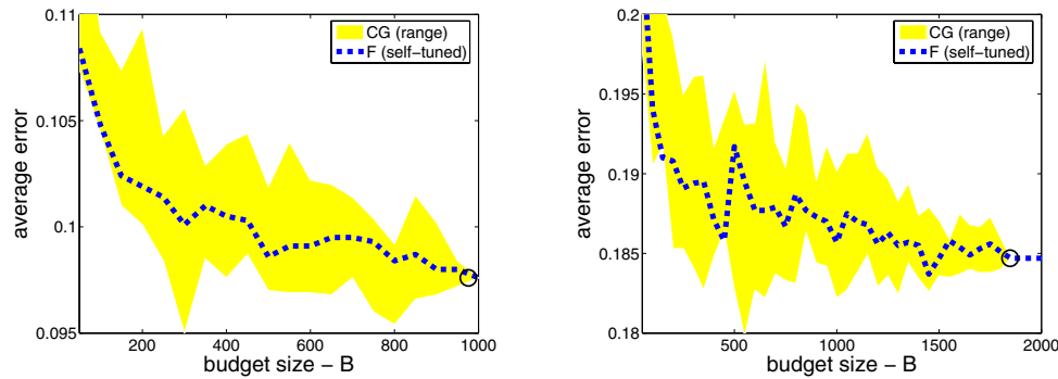
FIG. 7. The online error of the self-tuned Forgetron and the CG algorithm on a single dataset with 5% label noise (left) and on a single dataset with 10% label noise. For the CG algorithm, the range of online errors over 10 runs is given.
