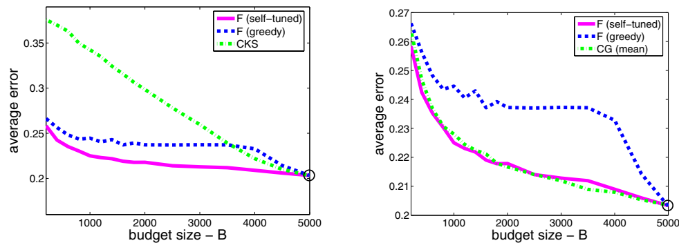
FIG. 5. The average online error of different budget algorithms as a function of the budget B on the census-income (adult) dataset. The average error of the Perceptron and its budget requirements are marked with a circle.
