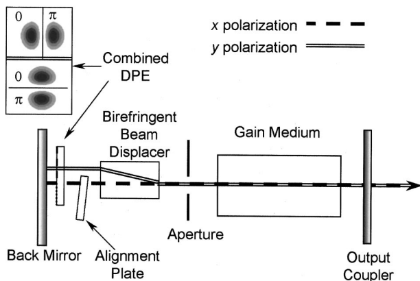
FIG. 2. Laser resonator configuration with a discontinuous phase element (DPE) for forming azimuthally or radially polarized beam.
