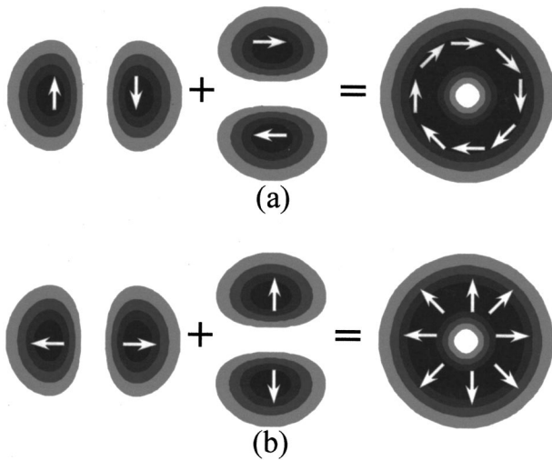
FIG. 1. Coherent superposition of two orthogonally polarized TEM_{01} modes to form azimuthally and radially polarized beams; (a) azimuthally ( \theta ) polarized doughnut beam; (b) radially ( r ) polarized doughnut beam.
