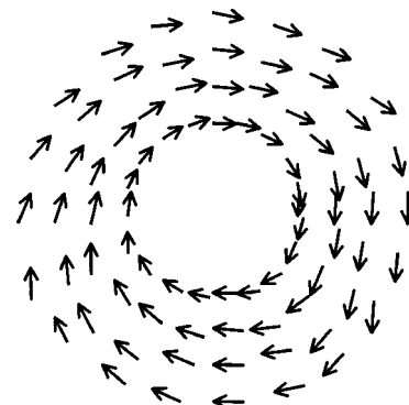
FIG. 4. Experimental plot of the space variant polarization directions of the emerging azimuthally polarized beam.
