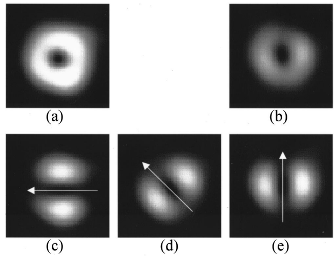
FIG. 3. Experimental intensity distributions of an azimuthally polarized beam that emerge from a Nd:YAG laser; (a) directly from the laser with no external elements; (b) after passing a horizontal \lambda/4 plate and a polarizer oriented at 45^\circ ; (c) after passing a polarizer oriented in the horizontal direction; (d) after passing a polarizer oriented at 45^\circ ; (e) after passing a polarizer oriented in the vertical direction.
