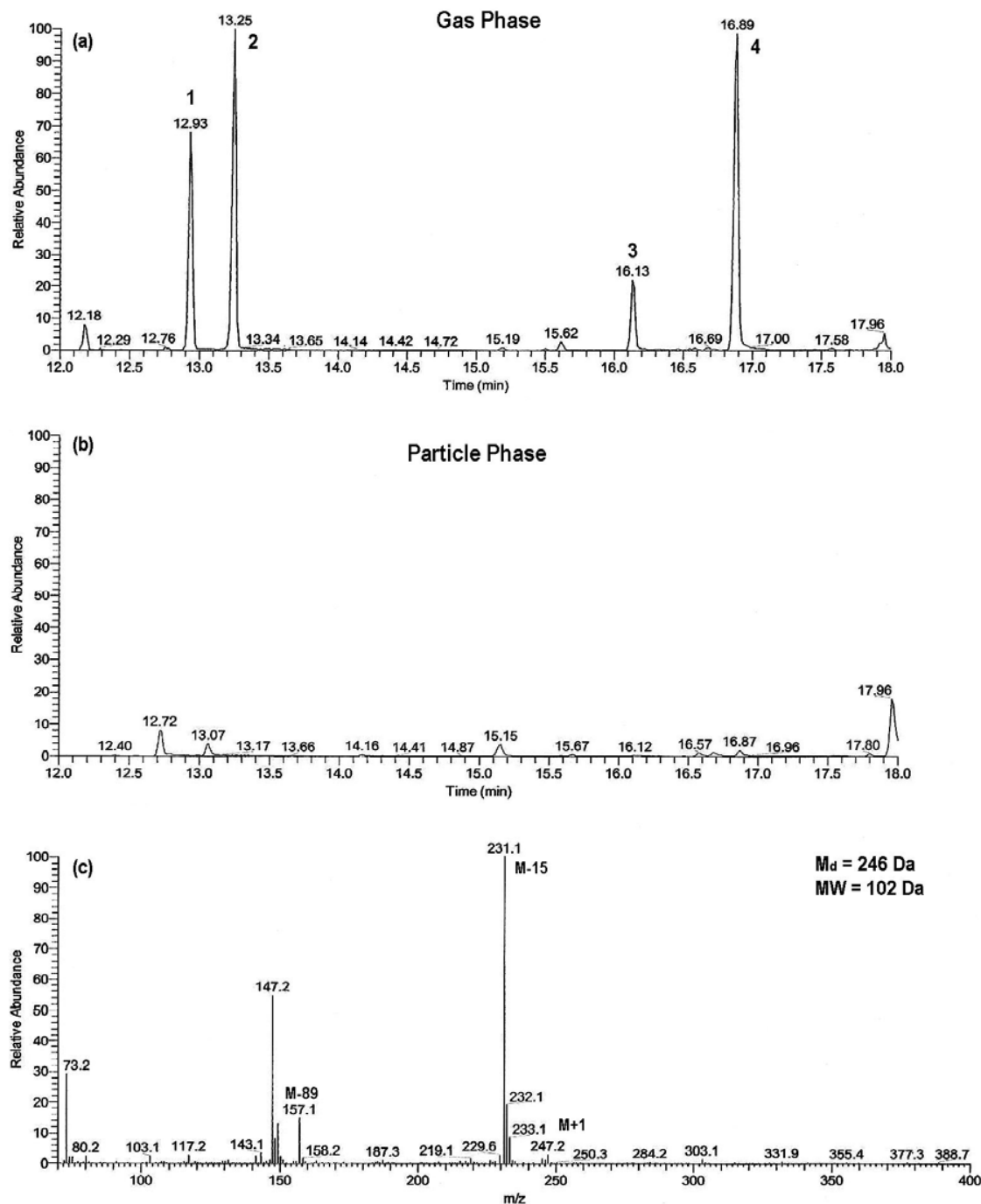
Fig. 2. Gas (a) and particle (b) phase chromatograms and mass spectrum (c); (Peak 1) of the butenediols in Experiment 2. For clarity in (a) and (b), the selected ion m/z 231 is shown.
