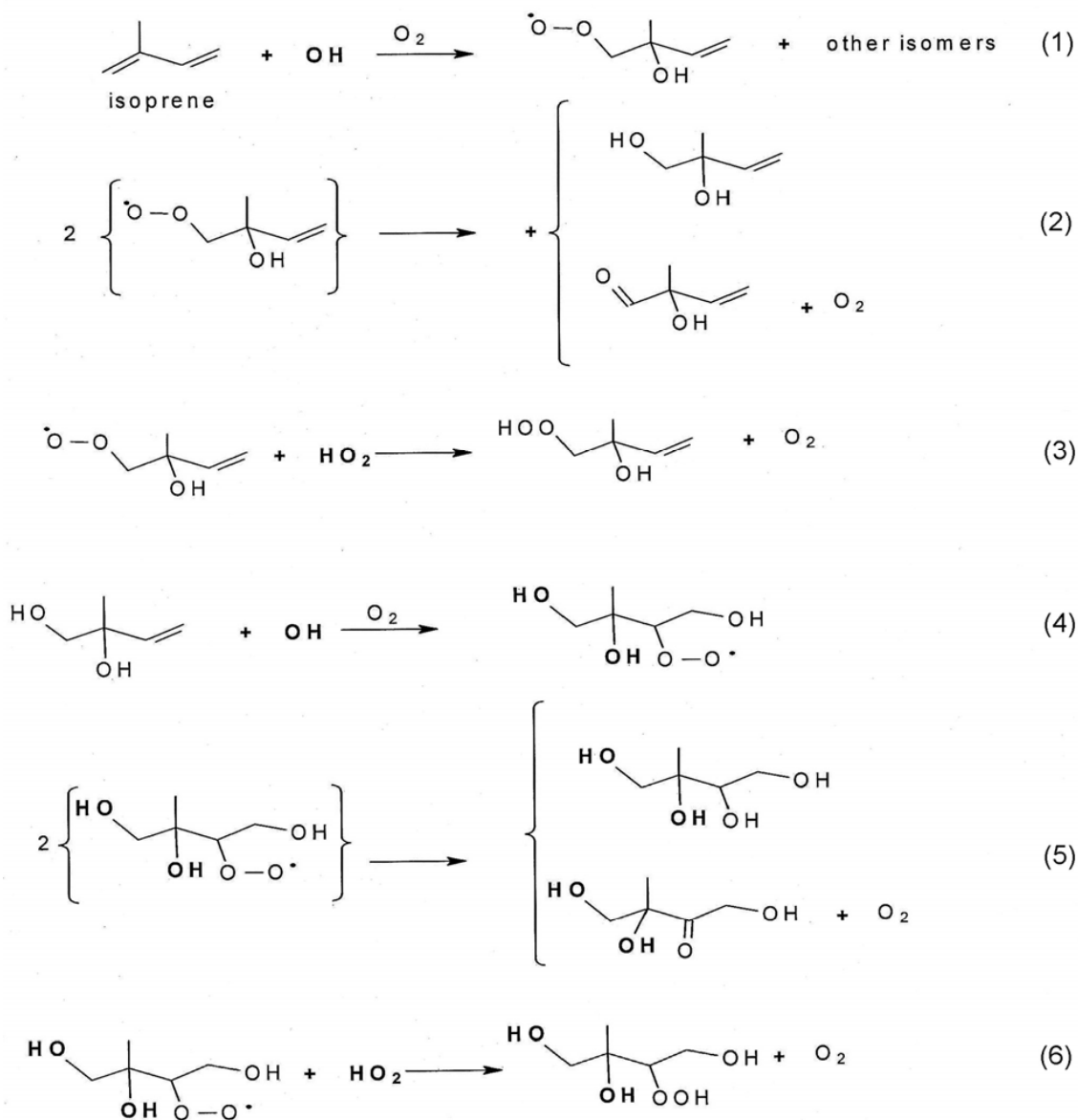
Scheme 1. Possible mechanism for the formation of the methyl tetrols in the absence of \text{NO}_x and acidic sulfate seed aerosol.
