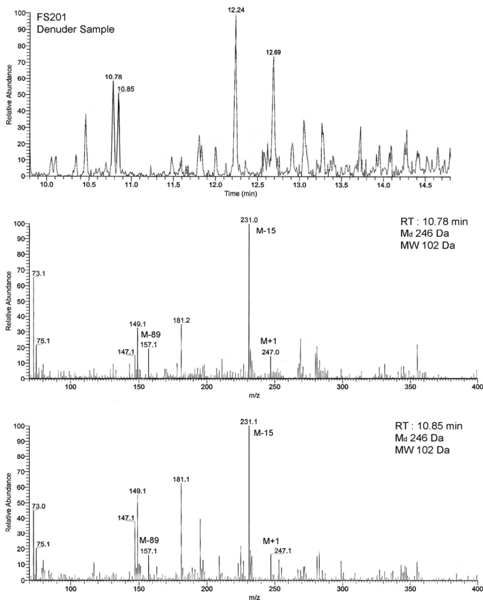
Fig. A1. Gas phase chromatograms and mass spectrum of the butenediols for Sample FS201 as described by Edney et al. (2003). The methyl butenediols are found at retention times of 10.78 and 10.85 min. For clarity, the selected ion chromatogram for m/z 231 is shown in the top panel. Experimental details and terminology used for the figure are the same as that in Edney et al. (2003).
