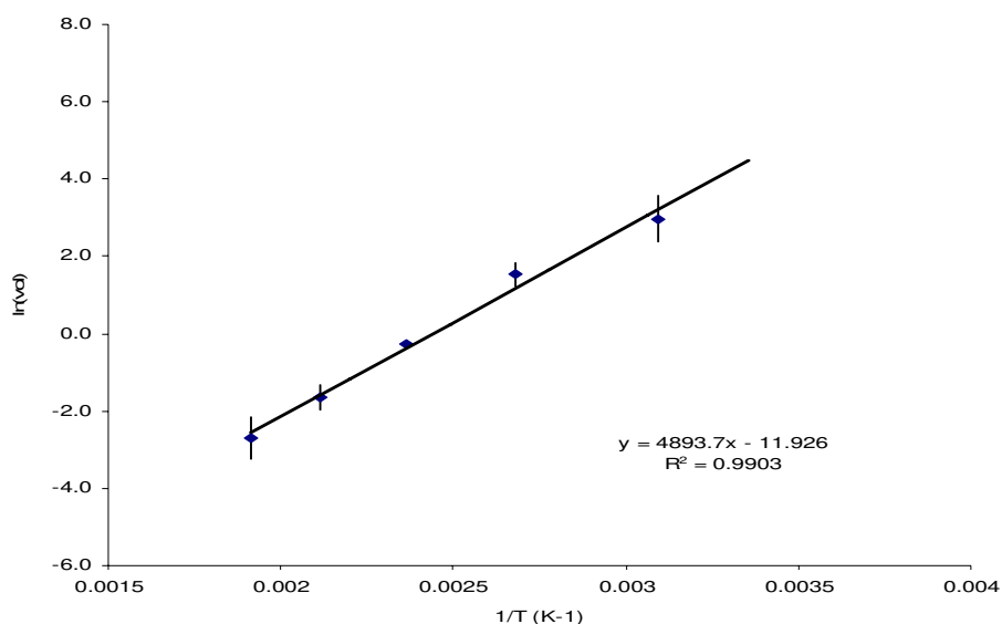
Fig. 1. Measured \Delta H_{\text{vap}}^{\text{eff}} of organic aerosol generated from the isoprene + OH reaction conducted in the absence of \text{NO}_x in Experiment 3.
