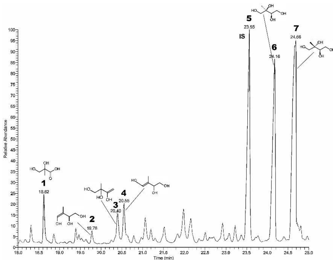
Fig. 3. Total ion chromatogram of filter extract of isoprene SOA formed in the absence of \text{NO}_x from Experiment 4. Identifications: (1) 2-methylglyceric acid; (2) cis -2-methyl-1,3,4-trihydroxy-1-butene; (3) 3-methyl-2,3,4-trihydroxy-1-butene; (4) trans -2-methyl-1,3,4-trihydroxy-1-butene; (5) Internal standard ( cis -ketopinic acid); (6) 2-methylthreitol; (7) 2-methylerythritol.
