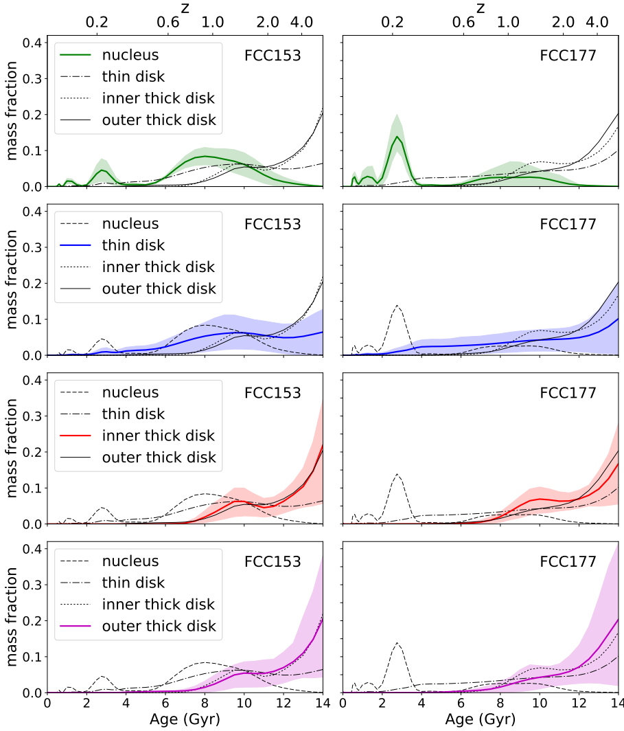
Fig. 7. SFH of the structural components of FCC 153 ( left column ) and FCC 177 ( right column ) defined in Fig. 6. The average mass fraction is displayed on the vertical axis. The average was calculated on the different spatial bins and was weighted with the mass in each one of them. This mass fraction is normalized to the total mass of the component. In each panel, only one component is represented in a specific color (green for the nucleus, blue for the thin disk, and red and purple respectively for the inner and the outer thick disk). For the colored component, 1\sigma uncertainties, calculated as 16% and 84% percentiles of the spatial-bin distribution, are represented as shades of the same color. The SFH of the rest of components are plotted in black, with different line styles, in each panel. As reference, the redshift scale on top of each column indicates the epoch when stars of a given age were born. The correspondence between redshift and age was approximated with Eq. (2) in Carmeli et al. (2006).
