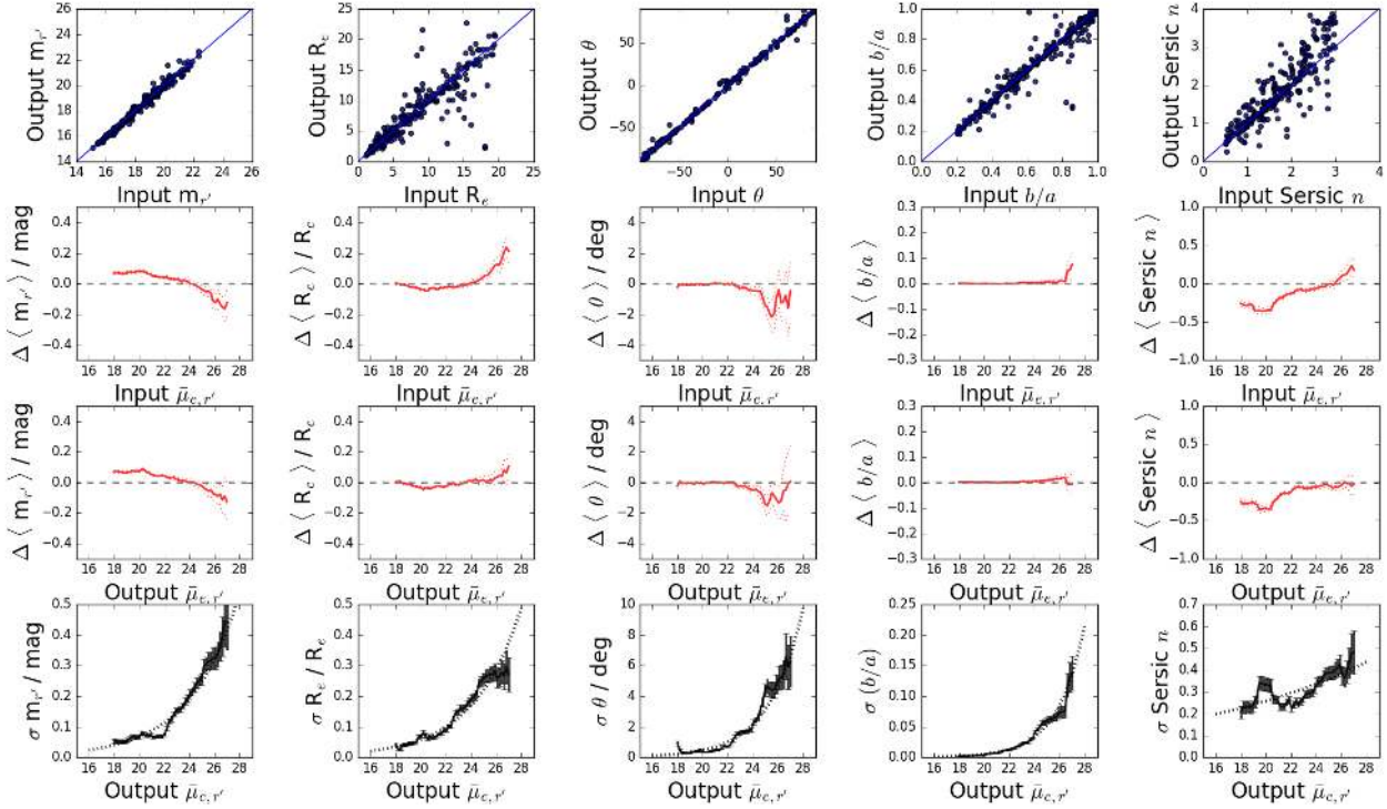
Fig. 14. Top row panels: comparison of the input structural parameters of the mock galaxies to the values measured by our photometric pipeline. The shown parameters are apparent magnitude ( m_r' ), effective radius in arcsec ( R_e ), position angle ( \theta ), axis ratio ( b/a ), and Sérsic index ( n ), and the blue diagonal lines represent the 1:1 ratio. Second and third row panels: mean differences between the input and output parameters (input – output) as a function of their input and output mean effective r' -band surface brightness, \bar{\mu}_{e,r'} , respectively. Bottom row: standard deviations of the input – output parameter differences as a function of the input mean \bar{\mu}_{e,r'} . The dotted lines in the bottom row panels show the fits to the standard deviations as defined in Eq. (10).
