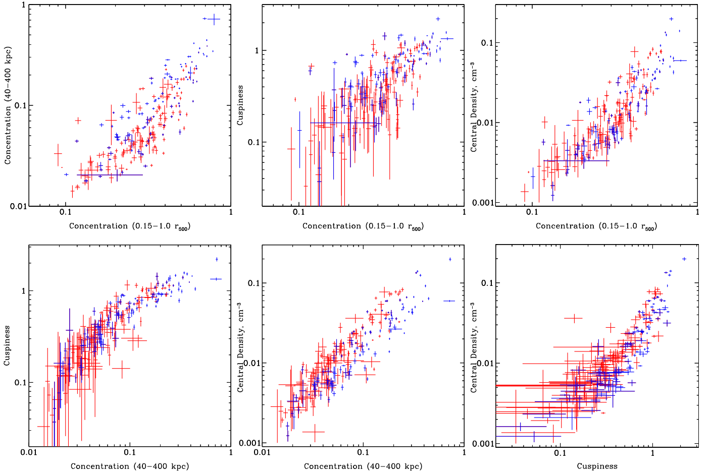
Figure 6. Top left: concentration parameter in the 40–400 kpc range ( C_{SB4} ) vs. concentration parameter in the 0.15–1.0 r_{500} range ( C_{SB} ). Top center: cuspsiness ( \delta ) vs. concentration parameter in the 0.15–1.0 r_{500} range ( C_{SB} ). Top right: central density ( n_{core} ) vs. concentration parameter in the 0.15–1.0 r_{500} range ( C_{SB} ). Bottom left: cuspsiness ( \delta ) vs. concentration parameter in the 40–400 kpc range ( C_{SB4} ). Bottom center: central density ( n_{core} ) vs. concentration parameter in the 40–400 kpc range ( C_{SB4} ). Bottom right: central density ( n_{core} ) vs. cuspsiness ( \delta ). The ESZ sample is in red and the X-ray sample is in blue. This figure shows the strong correlation between different metrics, whose correlations are quantified in Table 2.
