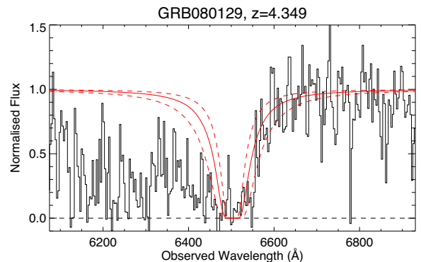
Figure A3. Fit of the red wing of Ly \alpha for the GRB 080129 VLT/FORS1 spectrum.
