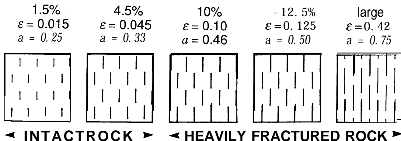
Figure 1. Schematic realization of percentage differential shear-wave velocity anisotropy in terms of crack density, \epsilon ; average normalized crack radius, a , for the values in Table 3. The panels represent approximate 2-D cross-sections through the cracked rocks.
