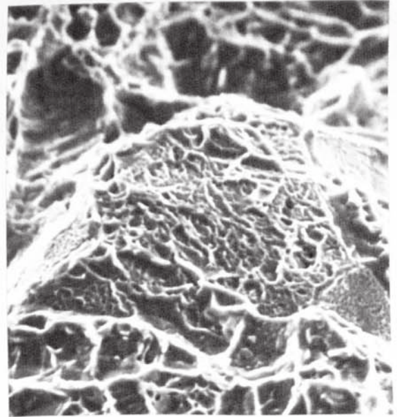
(b) Dimpled and flatter fracture 1200°C
