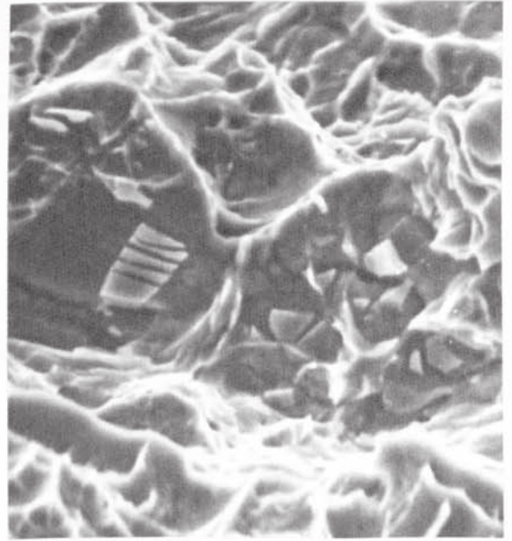
(b) Inclusion in the fracture. x 2500
