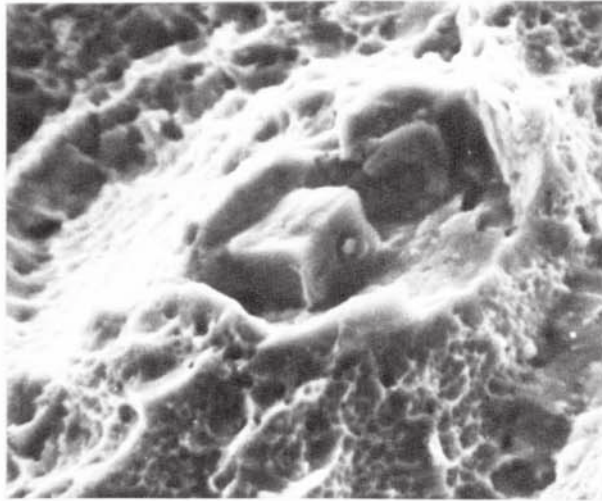
(a) Cuboid \text{Ti(CN)}
