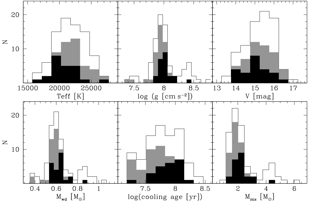
Fig. 1. Fundamental properties of the DA stars observed in this HST/COS far-ultraviolet spectroscopic survey. From top left to bottom right: effective temperature and surface gravity (Sect. 3), V-band magnitude, white dwarf mass and cooling age computed from T_{\text{eff}} and \log g using the cooling models of Fontaine et al. (2001), and the main-sequence progenitor mass computed from M_{\text{wd}} and the initial-to-final mass relation of Kalirai et al. (2008). The full sample is indicated by the outlined histogram. 48 white dwarfs where at least photospheric Si has been detected are shown with the filled histograms, of which 23 must be currently accreting (black). The remaining 25 (grey) have Si abundances consistent with support from radiative levitation alone, and have very likely accreted in the recent past (Sect. 9.1).
