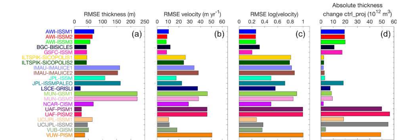
Figure 5. (a–c) Error estimate of model output at the end of the historical run compared to observations. (a) Root mean square error (RMSE) of ice thickness compared to observations (Morlighem et al., 2017). RMSE of the horizontal velocity magnitude (b) and the logarithm of the horizontal velocity magnitude (c) compared to observations (Joughin et al., 2016). The diagnostics have been calculated for grid cells subsampled regularly in space to reduce spatial correlation; we show median values for different possible offsets of this sampling. (d) Absolute thickness change in experiment ctrl_proj integrated over the model grid.
