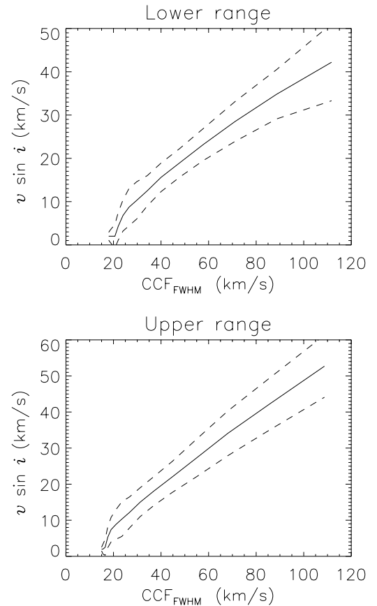
Fig. 6. The continuous line describes the relations between v \sin i and the CCF_{\text{FWHM}} used to derive v \sin i from the lower ( top panel ) and upper ( bottom panel ) wavelength range for the stars observed with the 580 set-up. Dashed lines describe the same relations plus/minus the error bars.
