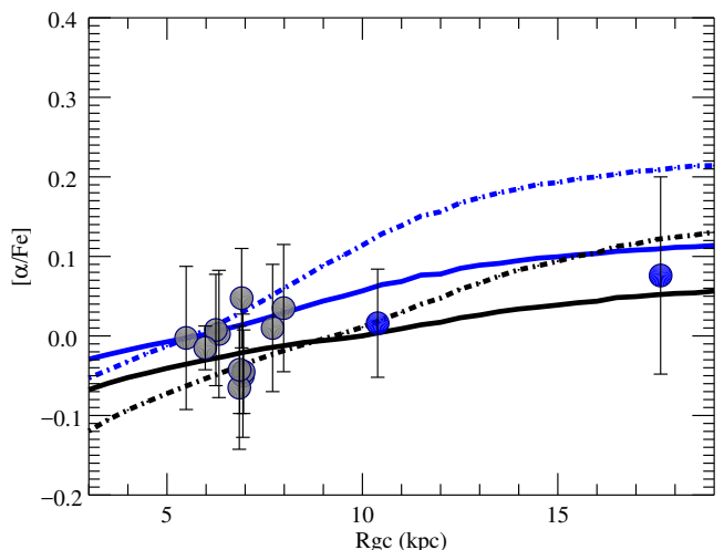
Fig. 8. Global \alpha -enhancement: [\alpha/\text{Fe}] vs. R_{\text{GC}} in the open cluster observations (colour coded by age as in Fig. 6) and in the K15-improved model (continuous lines, black at the present time and blue 5 Gyr ago). For comparison, the evolution of [\text{O}/\text{Fe}] vs. R_{\text{GC}} is shown (dashed-dotted lines, black at the present time and blue 5 Gyr ago).
