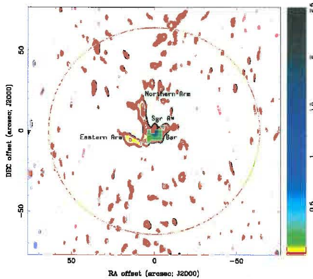
Fig. 2. Three-mm map of the mini-spiral region at resolution 2.68'' by 1.71'' (P.A= 20.7^\circ ). The green circle marks the HPBW. Contour levels are 0.02, 0.03, 0.04, 0.05, 0.1, 0.6, 0.9, 1.2, 1.5, and 2.5 Jy/beam.
