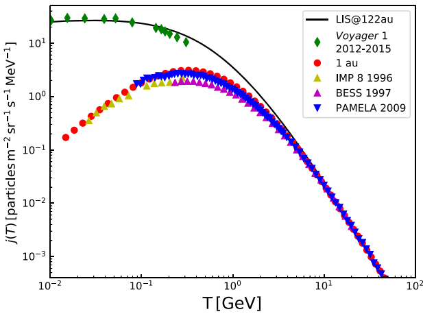
Figure A1. Differential intensity of Galactic cosmic rays as a function of kinetic energy. The solid black line represents a model fit of the Voyager 1 data (the green diamonds) for the LIS at 122 au that are the values used at the spatial outer boundary (122 au). The red dots represent our simulation results for 1 au. The yellow, magenta, and blue triangles are the IMP 8, BESS, and PAMELA observations, respectively.
