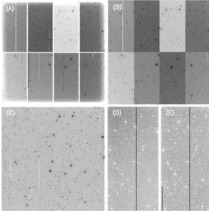
Fig. 1. Pre-reduction steps for WFI V -band data: (A) raw data, (B)&(D) debiased and flatfielded data (C)&(E) superflattened data. Taken from Erben et al. (2005).
