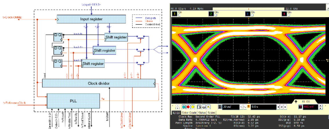
Figure 3. Serializer block diagram (left) and eye-diagram (right).
