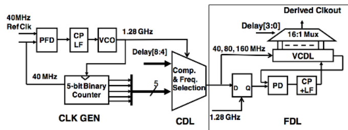
Figure 5. Phase shifter block diagram.
