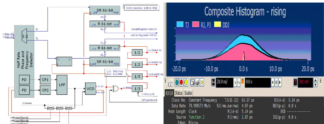
Figure 4. De-serializer block diagram (left), recovered clock jitter (right).
