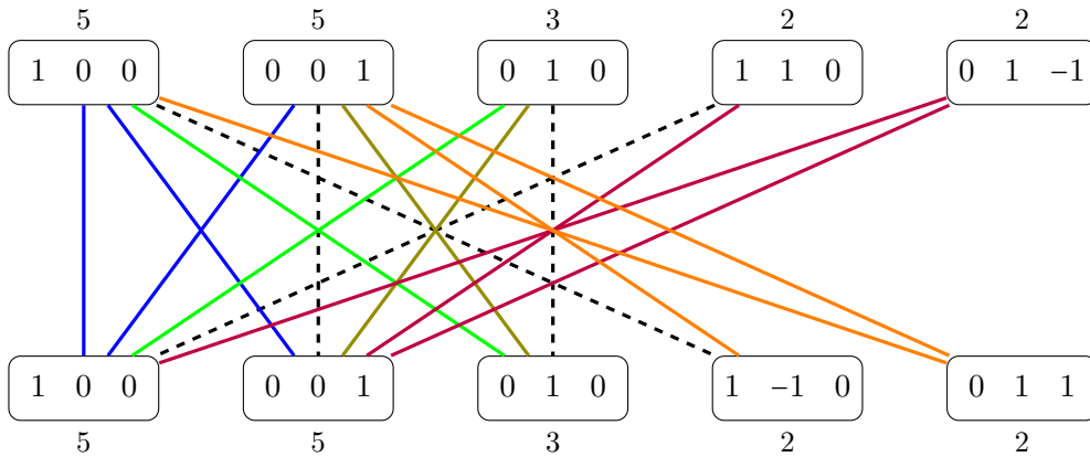
FIGURE 6. Pairing graph of decomposition \mathcal{S}_{\mathbb{Z}_4 \times \mathbb{Z}_3}
