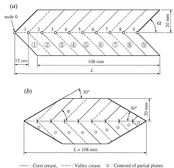
Figure 7. Double parallelogram model (a) (model 1), and double trapezium model (b) (model 2) used for numerical simulations. (a) A_0=4320 mm 2 , vein angle \alpha=15^\circ, 30^\circ, 45^\circ, 60^\circ, 75^\circ, 85^\circ . (b) A_0=2934 mm 2 , vein angle \alpha=30^\circ, 45^\circ, 60^\circ, 75^\circ, 85^\circ .
