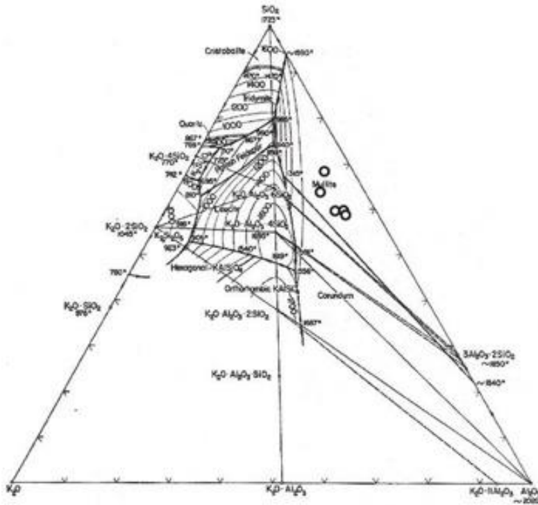
Figure 19a. Projection of the composition of Ile-Ife crucible fabrics (circles) into the ternary phase diagram for kaolinitic ceramic. The composition falls into an area with very high theoretical melting temperatures. Actual melting temperatures would be somewhat lower due to the presence of minor oxides, primarily iron oxide, working as fluxes. See table 5a for actual data.
