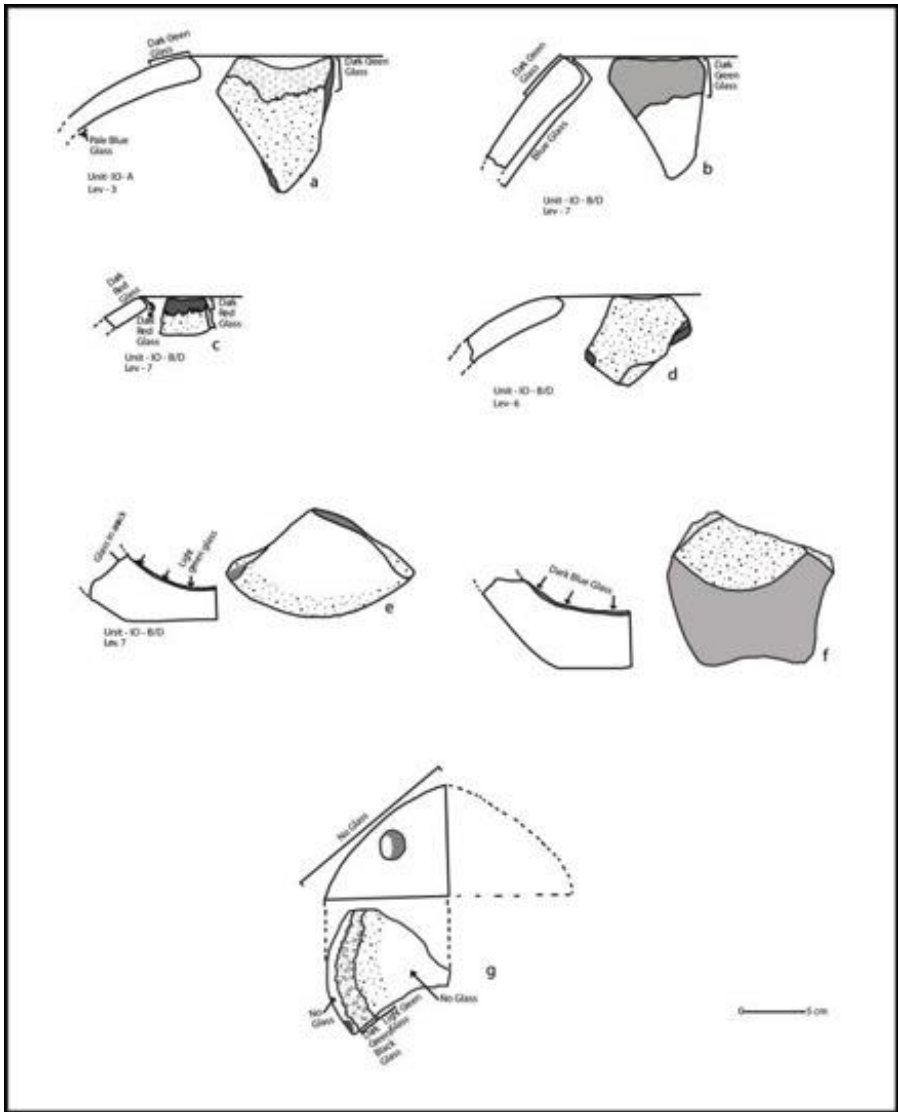
Figure 8. Sample profiles of Ile-Ife glass crucible fragments (Rim a-d; base e & f; lid g) (Lettering to be improved)
