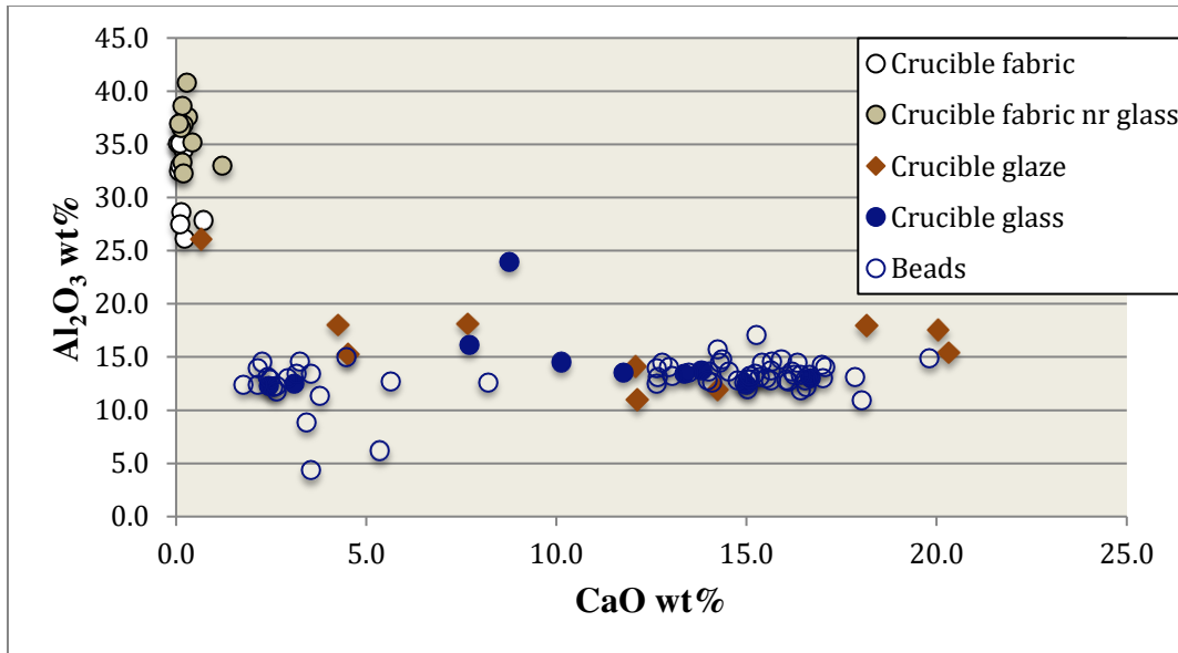
Figure 16. Alumina vs lime contents in analyzed crucible segments. The lime and alumina content of the crucible glaze matches the composition of the glass within the crucibles and also the glass beads.
