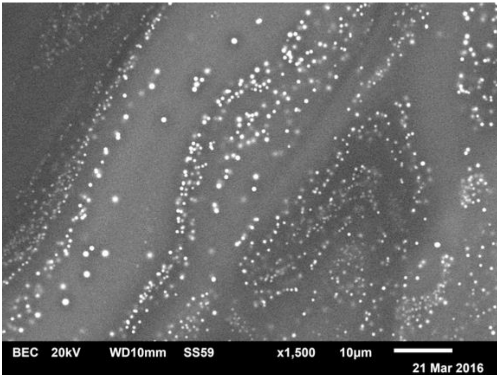
Figure 22. BSE image of copper particles in the inner red glass of a crucible from Igbo Olokun (sample IF0077). The lighter area in form of swirls is an indication of incomplete mixing of the colorant, in this case, metallic copper, into the glass matrix.
