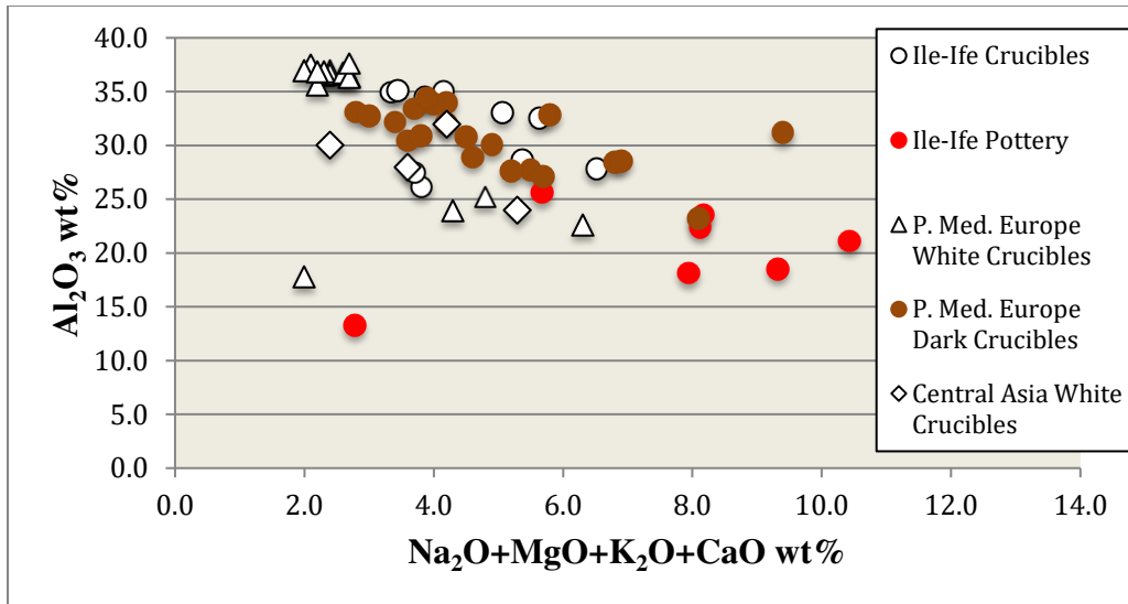
Figure 20. Comparison of alumina vs alkalis of Ile-Ife crucibles and Central Asian and post-medieval European crucibles (data from Martín-Torres and Rehren 2009; Central Asian data from Rehren and Papachristou 2003).
