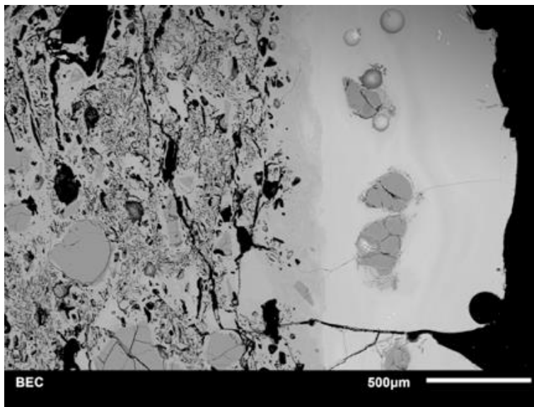
Figure 17. BSE image of the inner glass with quartz grains preserved in the glass matrix (light gray layer on the right). This, and the presence of swirls of different bulk composition (different gray shades in the glass) indicate that glass may have been made in these crucibles from raw materials, resulting in incomplete reaction and heterogeneous glass melt forming (sample IF0074).
