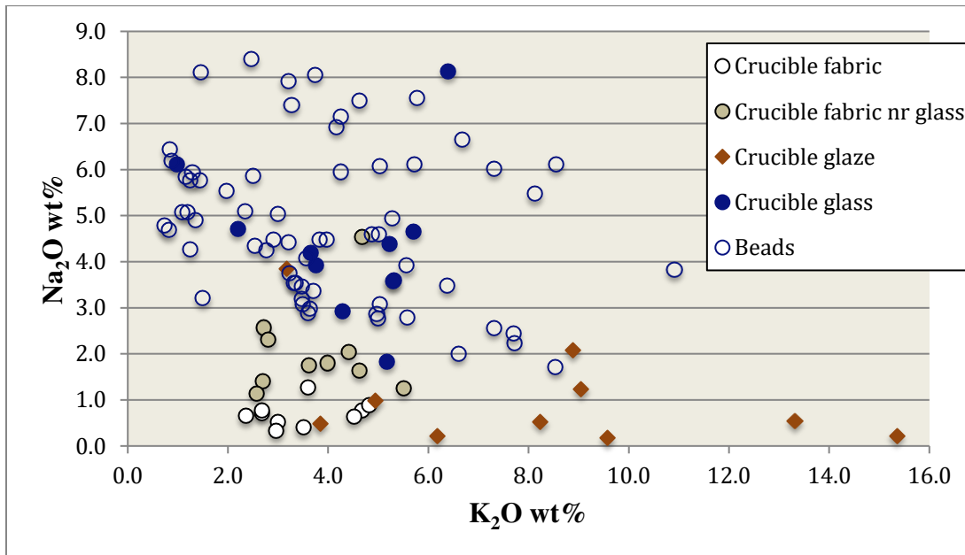
Figure 14. Comparing the soda vs potash contents in the major segments of the crucibles. Note how the crucible glass matches the glass beads, while the outer glaze is much richer in potash and lower in soda. The crucible fabric is low in both alkalis, indicating that it is not the source of the alkalis in either the glass or the glaze. Bead data from Babalola et al. (in press).
