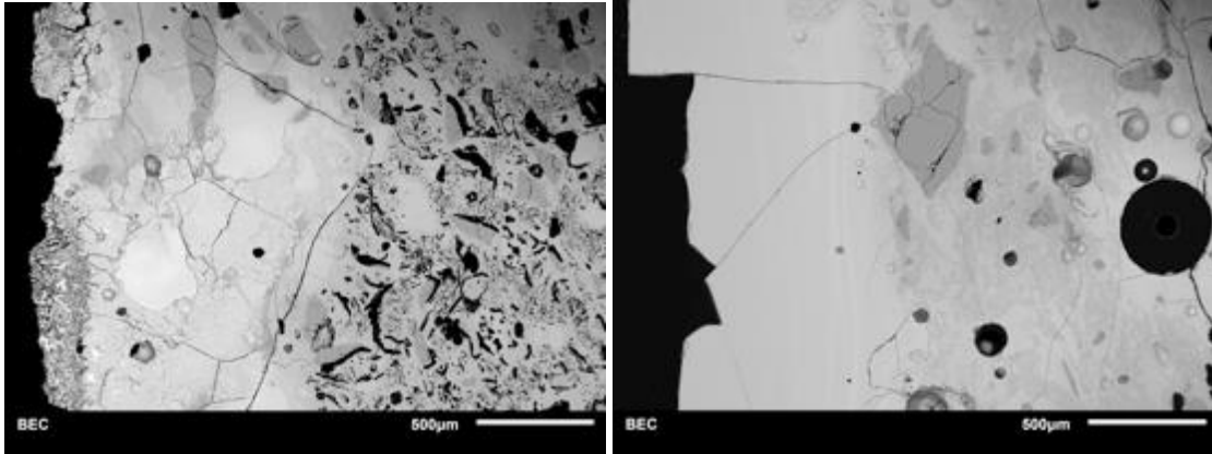
a b Figure 15. BSE image of examples of the matrix near the outer surface. a. Thin outer corroded glaze. Note the difference between the highly vitrified area of the fabric next to the glaze and the area farther from the glaze (sample F0074). b. Compositional analysis shows that the outer encrustation in this case is glass rather than glaze, indicating spillage of melted glass. Also note the highly vitrified area fronting the glaze (Sample IF0075).
