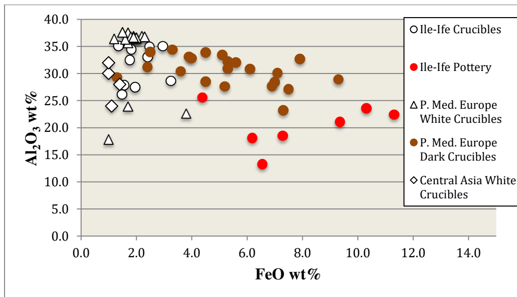
Figure 18. Comparison of alumina vs FeO content of Ile-Ife crucibles with the Ile-Ife domestic pottery and the post-medieval European crucibles (post-medieval European data from Martín-Torres & Rehren 2009; Central Asian data from Rehren & Papachristou 2003).
