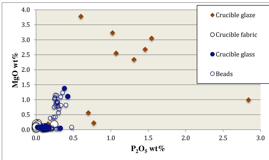
Figure 21. Comparing the magnesium vs phosphorus content of the areas in the crucibles with the glass beads, showing much higher values of both oxides in the outer glaze, typical for fuel ash.
