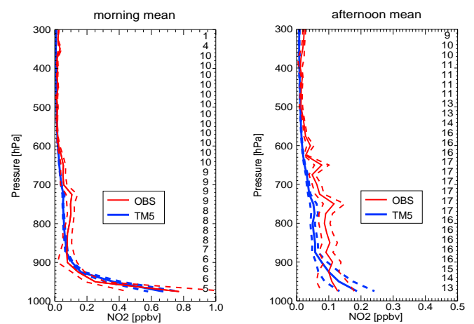
Fig. 11. Comparison of TM5 \text{NO}_2 profiles to aircraft measurements from the INTEX-B campaign over Mexico and the Gulf of Mexico during March 2006. Data is split into local times between 08:00–11:00 h (morning mean, left panel) and 11:00–16:00 h (afternoon mean, right panel). On the right side of the panels the number of available measurements in 25-hPa pressure bins is given. Dashed lines indicate the standard deviation of all individual observations and model results with respect to their means.
