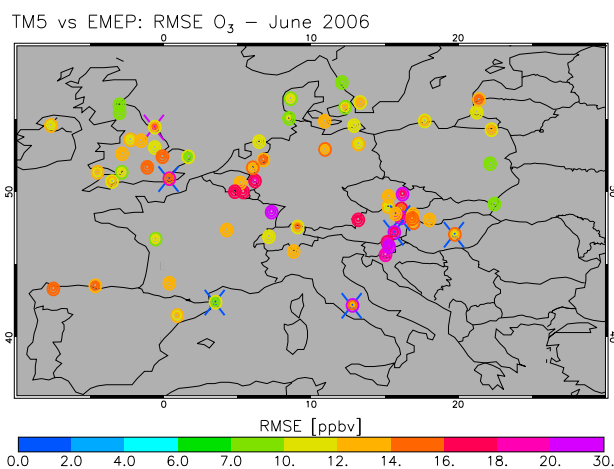
Fig. B2. Root mean square error (RMSE) of modeled surface ozone against hourly EMEP station data at stations below 800 m altitude. Outer circles: 3^\circ \times 2^\circ run, middle circles: 1^\circ \times 1^\circ , inner circles: 0.5^\circ \times 0.25^\circ . Blue crosses denote locations where an increase in resolution leads to a consistent reduction in RMSE with more than 2 ppbv for both zoom runs, compared to the 3^\circ \times 2^\circ run. Purple crosses denote a similar consistent increase in RMSE.
