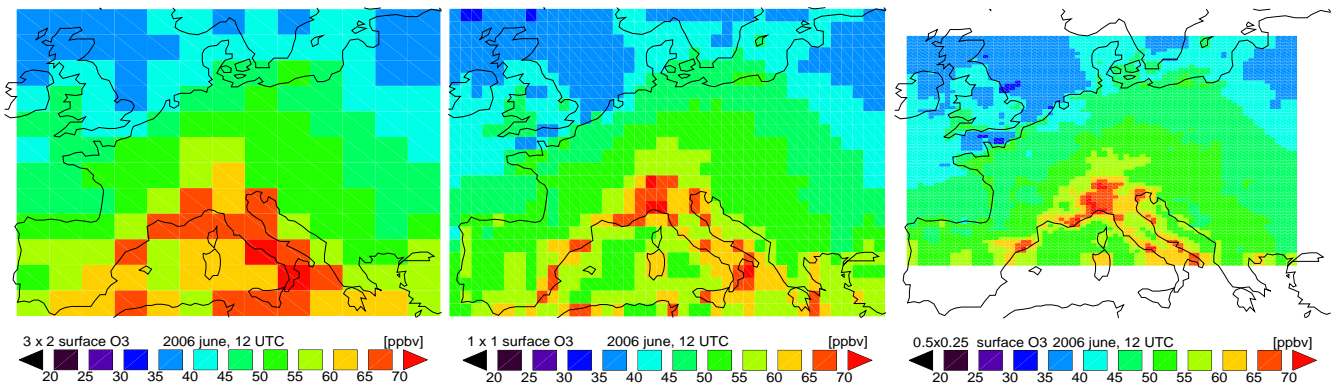
Fig. B1. Monthly mean surface ozone fields over Europe for June 2006 at 12:00 UTC, as simulated with increasing levels of zoom.
