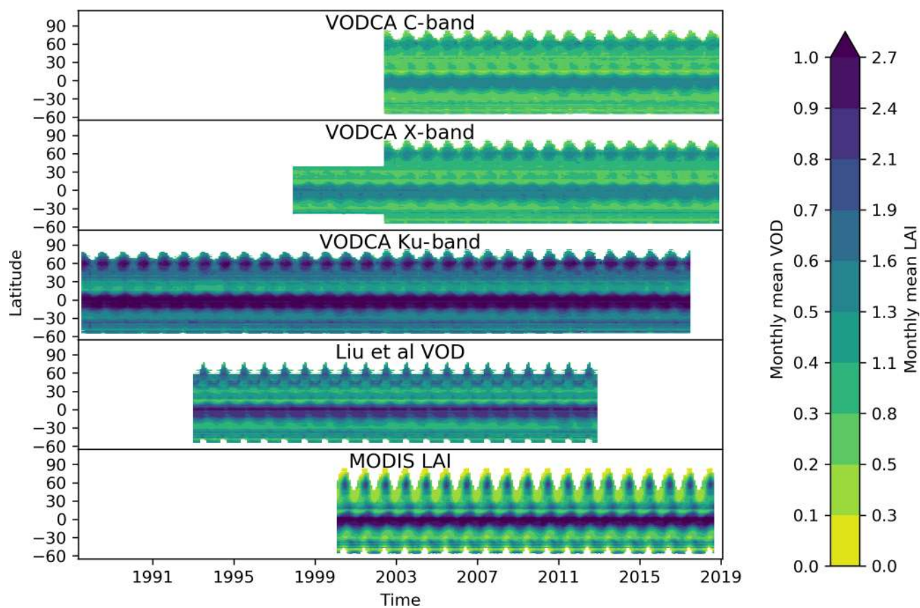
Figure 5. Hovmöller diagrams showing the monthly mean VOD per latitude for each band of VODCA and VOD_Liu and for LAI.
