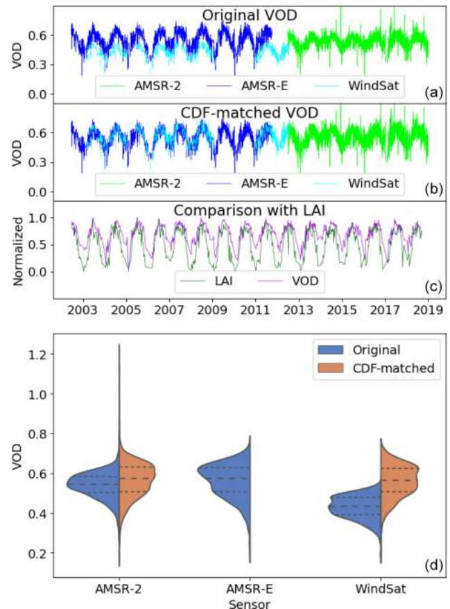
Figure 3. (a–c) Example X-band time series for a grid cell in Austria ( 15.125^{\circ} E, 48.125^{\circ} N, mostly farmland with about 20 % forest) at different processing steps. Time series of the original VOD data of all available sensors are shown in (a), the CDF-matched series in (b), and the final merged VOD (VODCA) together with MODIS LAI in (c). In (c) VOD and LAI are both normalized, and VOD is downsampled by moving average to match the temporal 8 d resolution of LAI. (d) Violin plot showing the effect of CDF matching on the statistical distribution of VOD.
