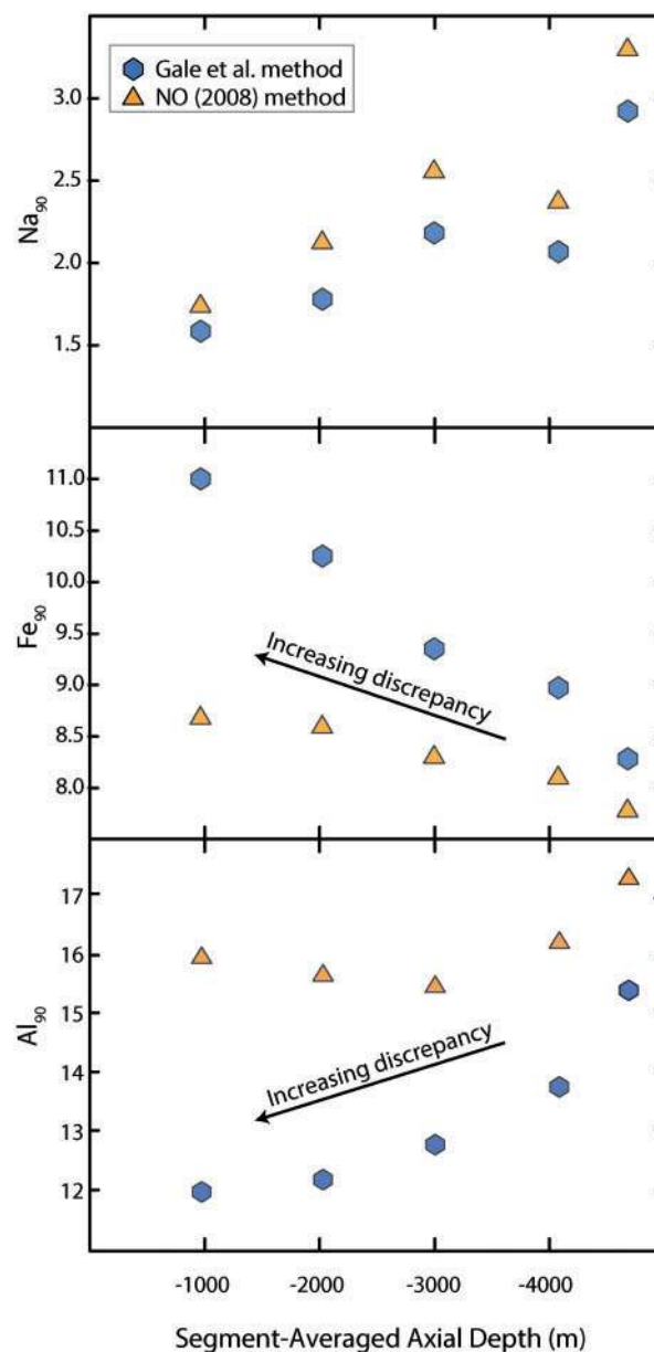
Fig. 19. Na_{90} , Fe_{90} and Al_{90} vs axial depth calculated for five segments over a large range of axial depths and chemical contents, comparing the different fractionation correction techniques in this study and in that of Niu & O'Hara (2008) [NO(2008)]. The axial depth shown is segment-averaged axial depth. It should be noted that the mistaken lowering of the high FeO contents when using the Niu & O'Hara (2008) polynomial causes increasing disparity of up to almost 2.5 wt % in the calculated Fe_{90} values. A similar disparity is seen in the calculated Al_{90} values. Because Na is an incompatible element much less sensitive to the exact crystallization sequence, the two studies track each other much more closely in Na_{90} .
