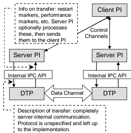
Figure 1: Globus GridFTP architecture
