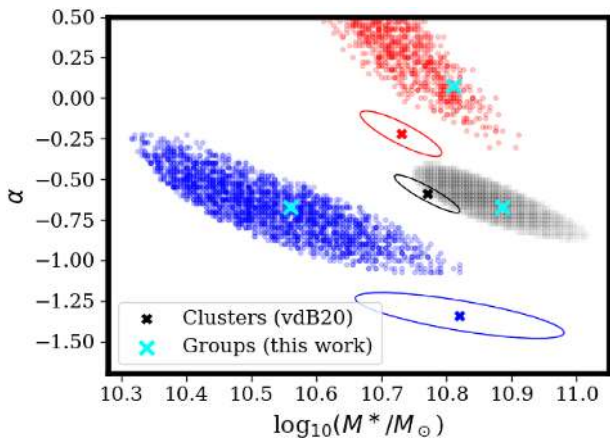
Figure 4. We show two of the Schechter function fit parameters for the 1 < z < 1.5 galaxy group population, for the total sample (black), the quiescent galaxies (red), and the star-forming galaxies (blue). Points represent draws of parameters within the 68 per cent confidence limits of the fits. The cyan crosses indicate the best-fitting parameters. The \alpha parameter for the quiescent population is effectively unbounded: high values of \alpha > 2 provide acceptable fits within 2\sigma . The crosses with solid ellipses represent the fit parameters and 68 per cent confidence limits for the massive cluster population at the same redshifts, from van der Burg et al. 2020.
