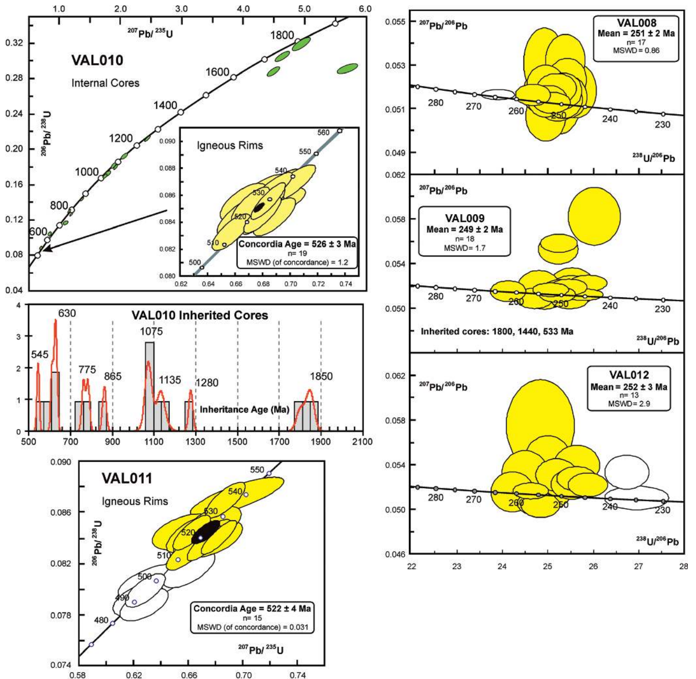
Fig. 3. New SHRIMP U–Pb data for samples from the Tardugno Granodiorite (data corrected for common Pb using measured ^{204}\text{Pb} ) and Yaminué complex granites (uncorrected data). White ellipses represent data omitted from age calculation.
