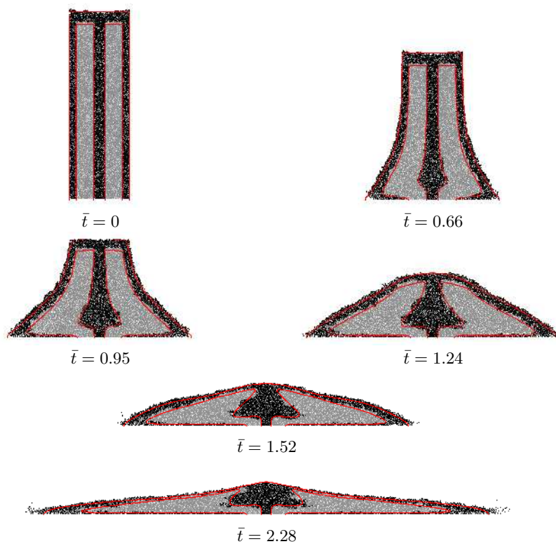
FIGURE 10. Comparison between the \mu(I) continuum model (red line) and contact dynamics simulations (grains) for an aspect ratio a = 6.26 at different times (non-dimensionalized by \sqrt{H_0/g} ). The parameters of the \mu(I) -rheology are \mu_s = 0.32 , \Delta\mu = 0.28 and I_0 = 0.4 (color online).
