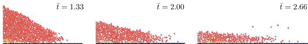
FIGURE 18. Snapshots of the flow front at \bar{t} = 1.33 , \bar{t} = 2.00 and \bar{t} = 2.66 for a discrete numerical simulation with aspect ratio a = 6.26 . Note the rough plane obtained by "gluing" grains.
