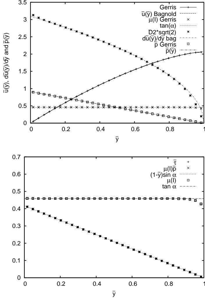
FIGURE 2. Comparison between (a) analytical and (b) computed (on a 32x32 grid) profiles for a single granular layer ( 0 < \bar{y} < 1 ) with the \mu(I) -rheology. The slope angle is \alpha = 0.43 , and \bar{d} = 1/25 . (a) analytical (2.16) and Gerris solution for the pressure, velocity and velocity gradient. (b) Comparison of shear stress \bar{\tau} = \bar{\eta}d\bar{u}/d\bar{y} (+), \mu(I)\bar{p} (x) and exact solution (dashed line); and comparison of the computed \mu(I) ( \square ) with the exact solution \tan\alpha (dot-dashed line).
