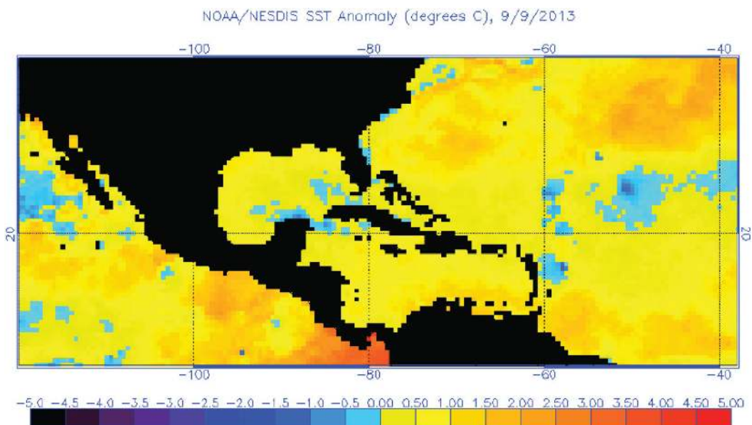
FIG. A1. Sea surface temperature anomaly ( ^{\circ}\text{C} ) for 9 Sep 2013. (Source: NOAA/NESDIS.)
