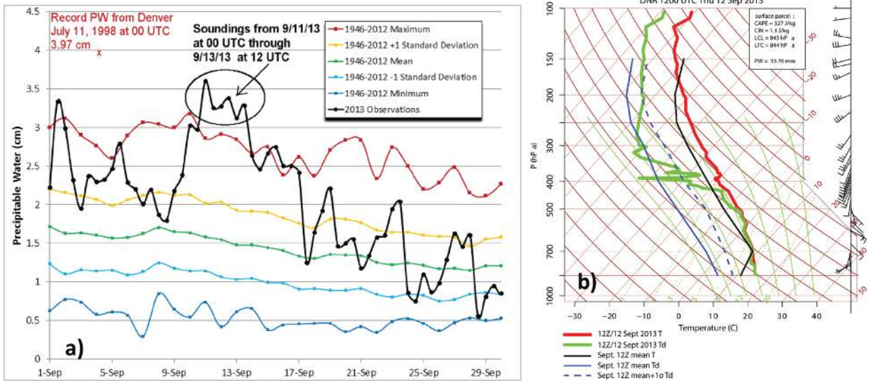
FIG. 5. (a) PW (in cm) from the surface to 300 hPa as measured from radiosondes in Denver. Plotted are the daily means, maxima, minima, and one standard deviation above and below the means for days in Sep based on climatological data from 1946 to 2012 for Sep. Also plotted are the values measured in Sep 2013 (in black). Six consecutive soundings from 0000 UTC 11 Sep to 1200 UTC 13 Sep set new single-day PW records. The all-time Denver PW record from 11 Jul 1998 is also plotted for reference. (b) Skew T - \log p diagram of the sounding from Denver at 1200 UTC 12 Sep 2013. The solid black line shows temperature, and the solid green line shows dewpoint at this time. The solid red line shows the mean 1200 UTC temperature for Sep, the solid blue line shows the mean 1200 UTC Sep dewpoint, and the dashed blue line shows the mean dewpoint plus one standard deviation. These mean and standard deviation calculations used observations from 1957 to 2012 and only mandatory levels. The 1200 UTC 12 Sep 2013 sounding was launched into cloud and precipitation, which is representative of the widespread moist upslope conditions in Colorado during 11–13 Sep but may not be representative of the conditions in cloud-free areas.
