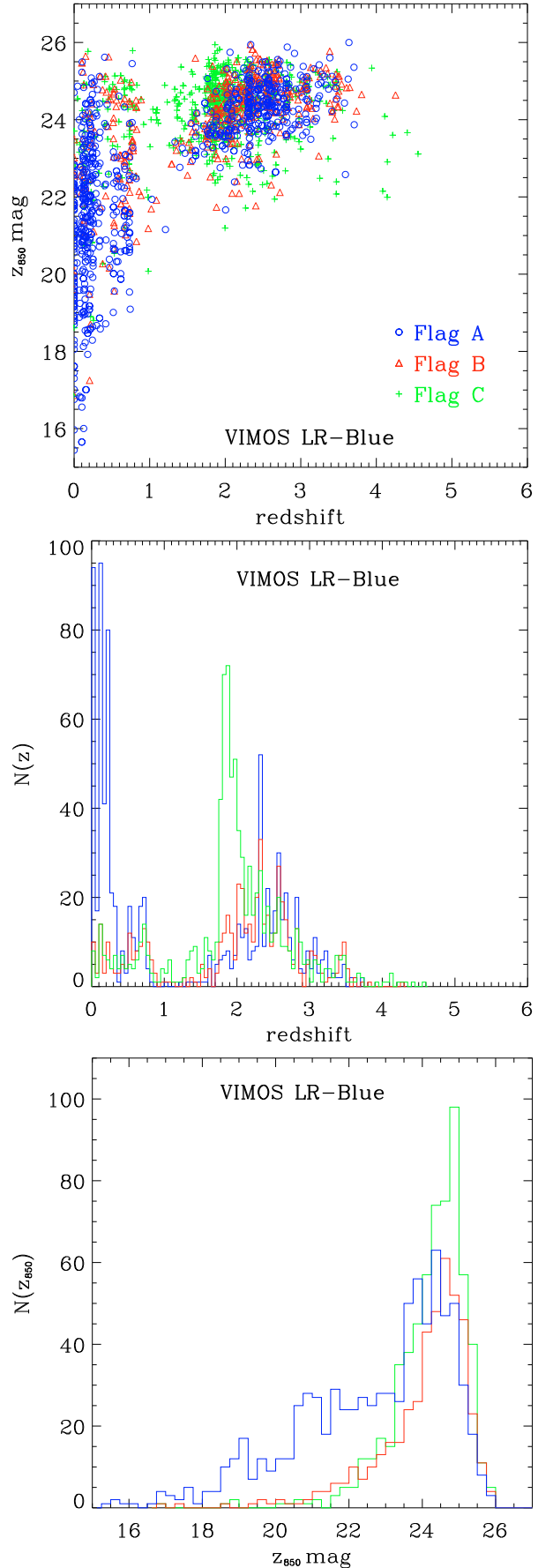
Fig. 7. VIMOS LR-Blue survey: GEMS z_{850} magnitudes versus redshift (upper panel), histogram of the redshift distribution (middle panel), and histogram of the z_{850} magnitude distribution (lower panel).
