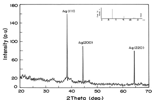
Fig. 3 The XRD pattern of Ag NPs
