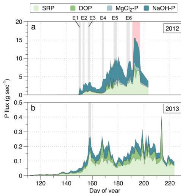
Figure 5. Time series of calculated phosphorus fluxes at (a) Leverett Glacier and (b) Kiattuut Sermia. Only “bioavailable” phosphorus fractions are shown (dissolved P phases plus MgCl_2 -P and NaOH-P). Dissolved fluxes are represented with green colors, and particulates fluxes with blue/grey colors. Fluxes are cumulative at each time point. Grey shaded areas in Figure 5a are indicative of outburst events (E) and in Figure 5b of a significant hydrological shift in the glacial drainage system (a spring event). The red shaded area in Figure 5a highlights the 2012 record melt event.
