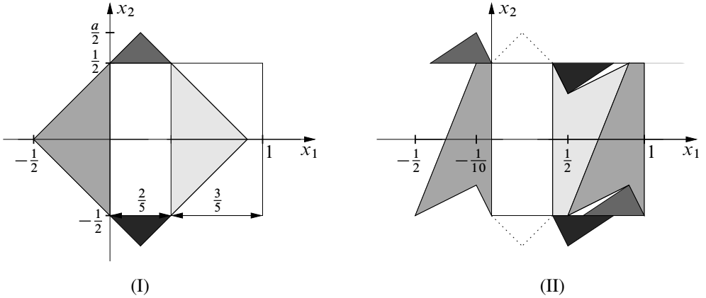
Figure 8: Filling \frac{49}{50} of T(1, 1) , schematically
