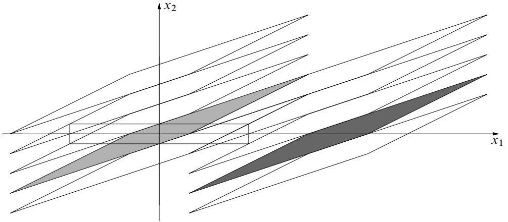
Figure 6: The tiling of \mathbb{R}^2(\mathbf{x}) by translates of P(k) (in the picture k = 3 ). The darker parallelogram is a translate of the lighter one by 2k^2 in the x_1 -direction. The rectangle marks the standard fundamental domain already depicted in Figure 5.
