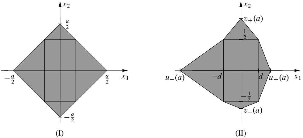
Figure 3: The diamond \diamond(a) and a distorted diamond
