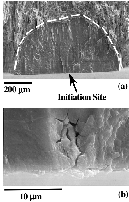
Figure 5. Fatigue crack/initiation.
